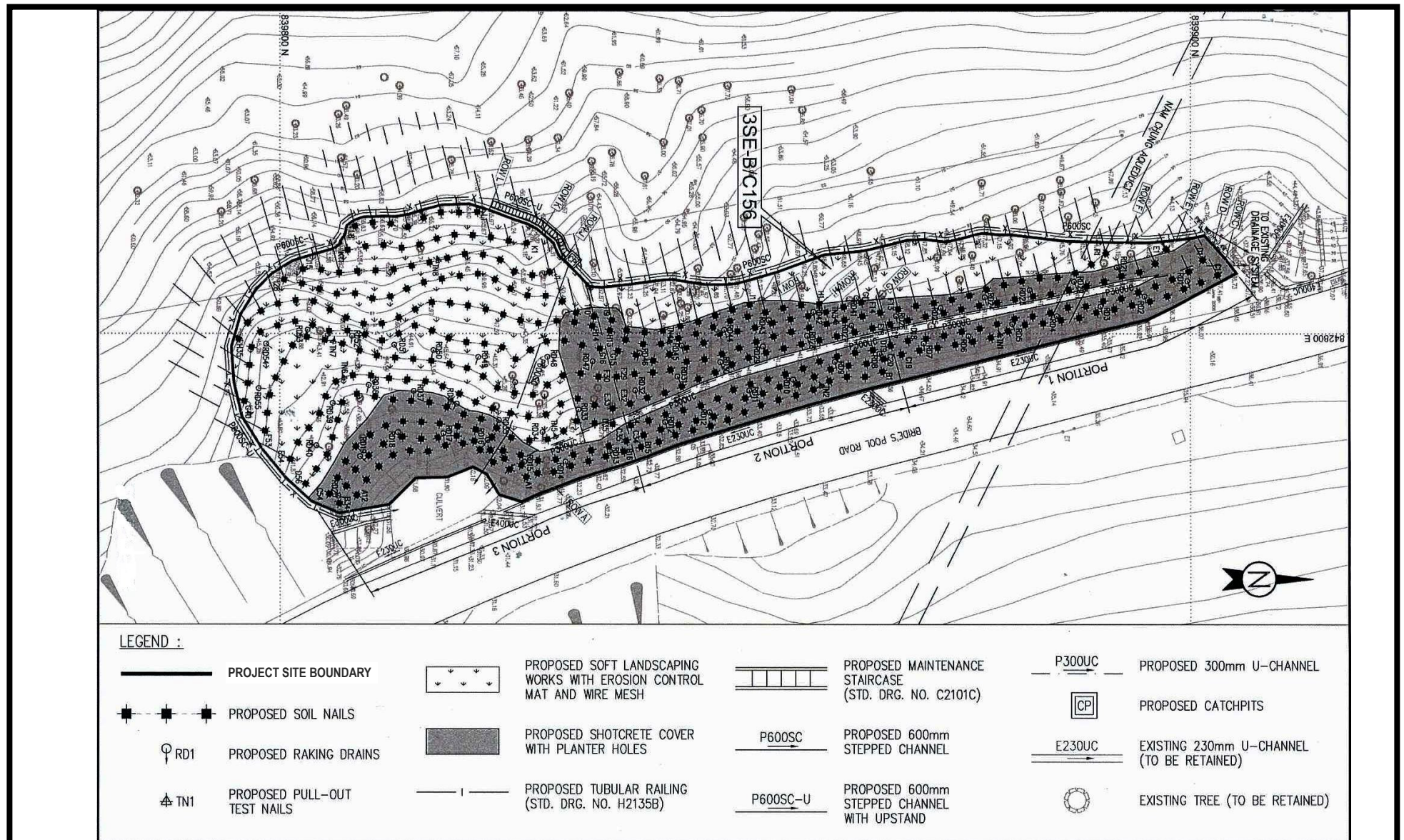
Figure 2 Landslip Preventive Works at Feature No. 3SE-B/C156 Along Bride's Pool Road, Near Chung Mei Plover Cove Reservoir, Tai Po (人造斜坡編號 3SE-B/C 156 的防止山泥傾瀉工程在大埔涌尾近船灣淡水湖，新娘潭路旁)
