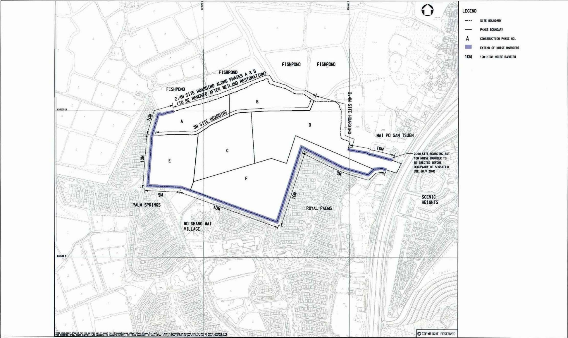
Figure 2 – Minimum Height Required for Proposed Noise Barriers and Site Hoardings 圖 2 - 建議隔音屏障及地盤圍板的起碼高度
