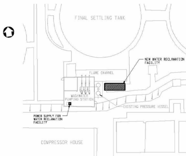
DETAIL A LOCATION PLAN OF WATER RECLAMATION FACILITY
