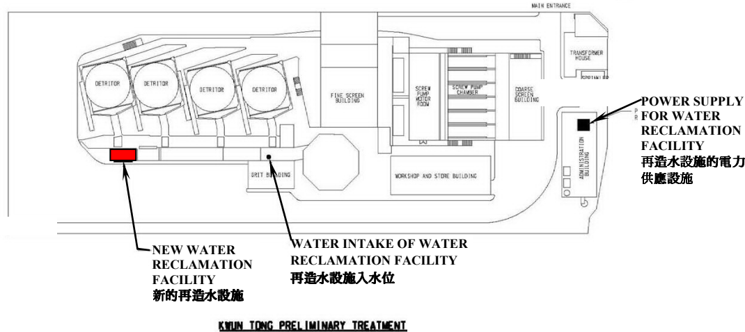
LAYOUT PLAN 平面圖 KWUN TONG PRELIMINARY TREATMENT WORKS 觀塘基本污水處理廠
