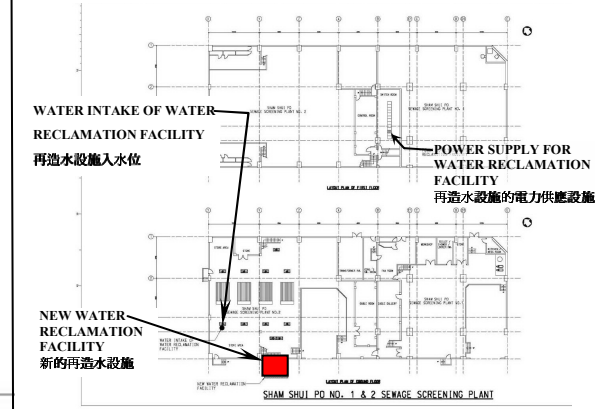
LAYOUT PLAN 平面圖 SHAM SHUI PO NO. 1 & 2 SEWAGE SCREENING PLANT 深水埗一期和二期污水隔篩廠
