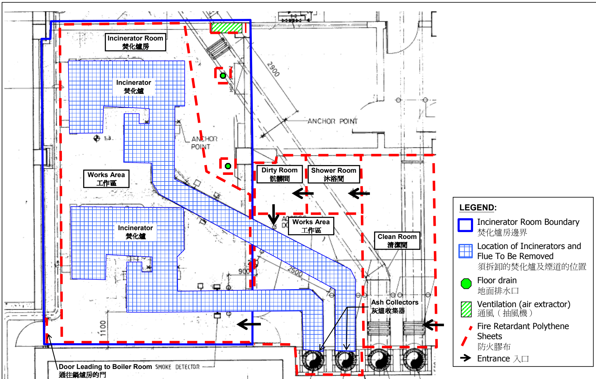
FIGURE 2: Floor Plan of the Incinerator Room
