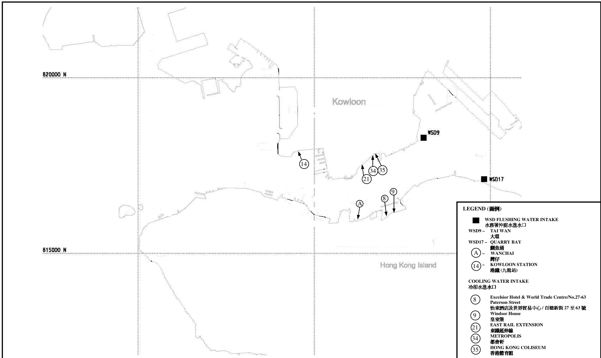
Figure 4: The Locations of Cooling Water Intake and WSD Flushing Water Intake
