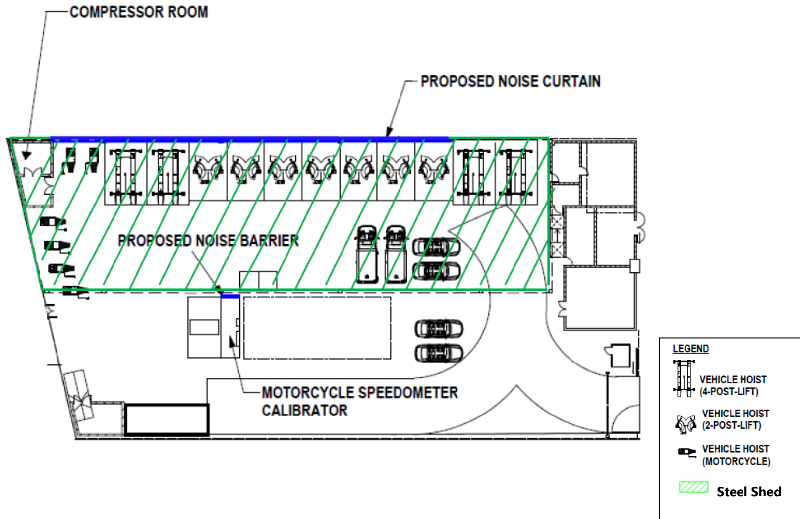
Figure 2: General Layout Plan
