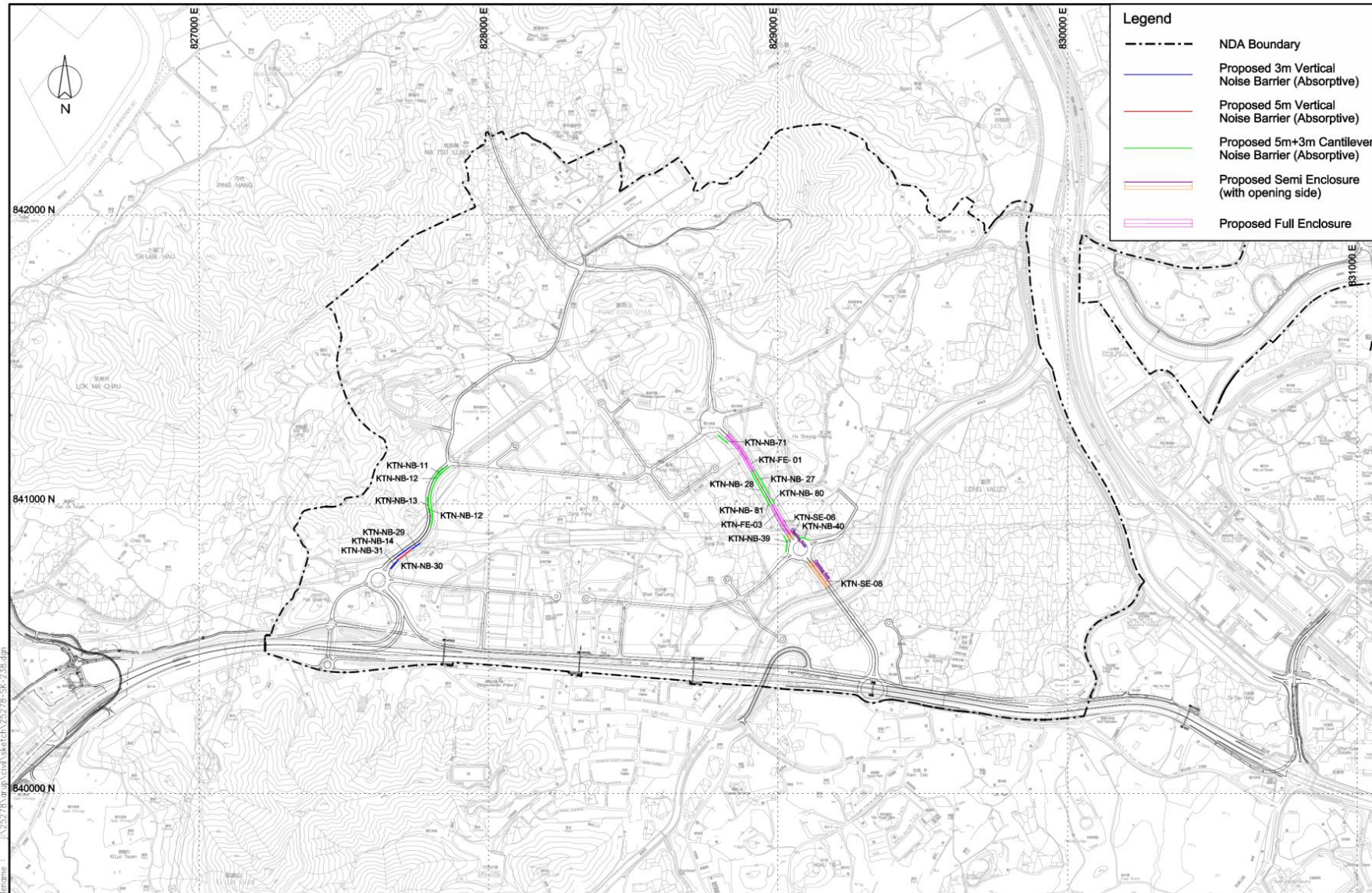
Project Title: Kwu Tung North New Development Area Road P1 and P2 and Associated New Kwu Tung Interchange and Pak Shek Au Interchange Improvement Figure 3: Location Plan for the Proposed Noise Barriers
