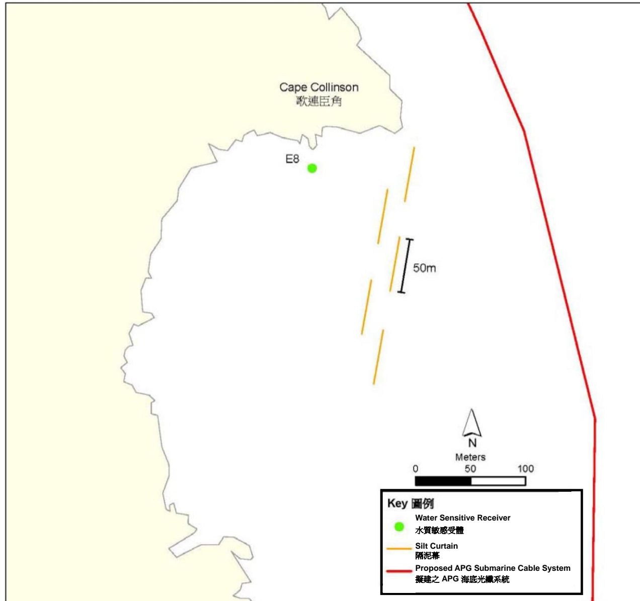
Project Title: Asia Pacific Gateway (APG) - Tseung Kwan O 工程項目名稱: Asia Pacific Gateway (APG) - 將軍澳 The Location of Silt Curtain for Water Sensitive Receiver (WSR) E8 為水質敏感受體 E8 的隔泥幕指示位置圖
