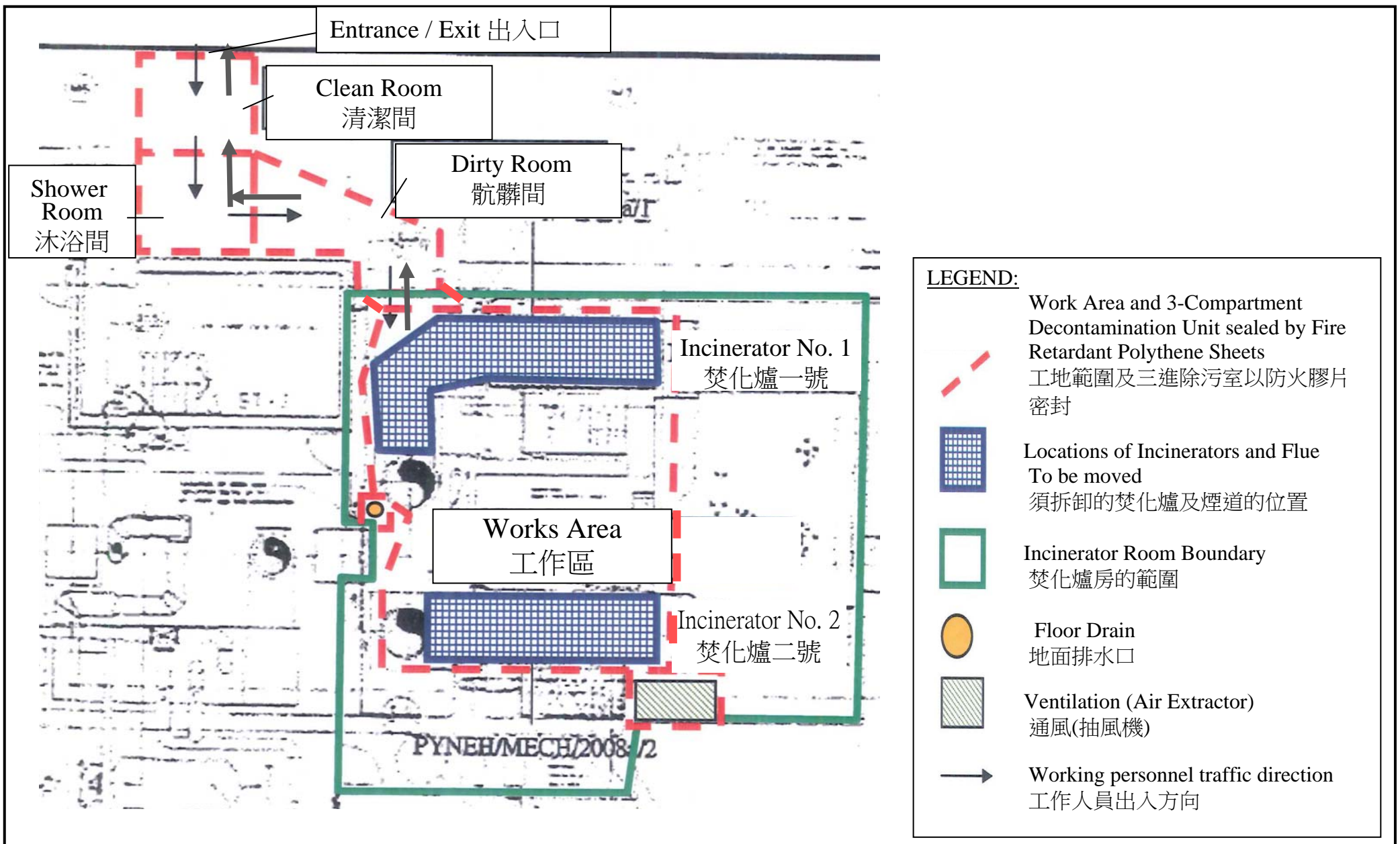
Figure 2: Floor Plan of the Works Area 圖 2: 工地樓面圖
