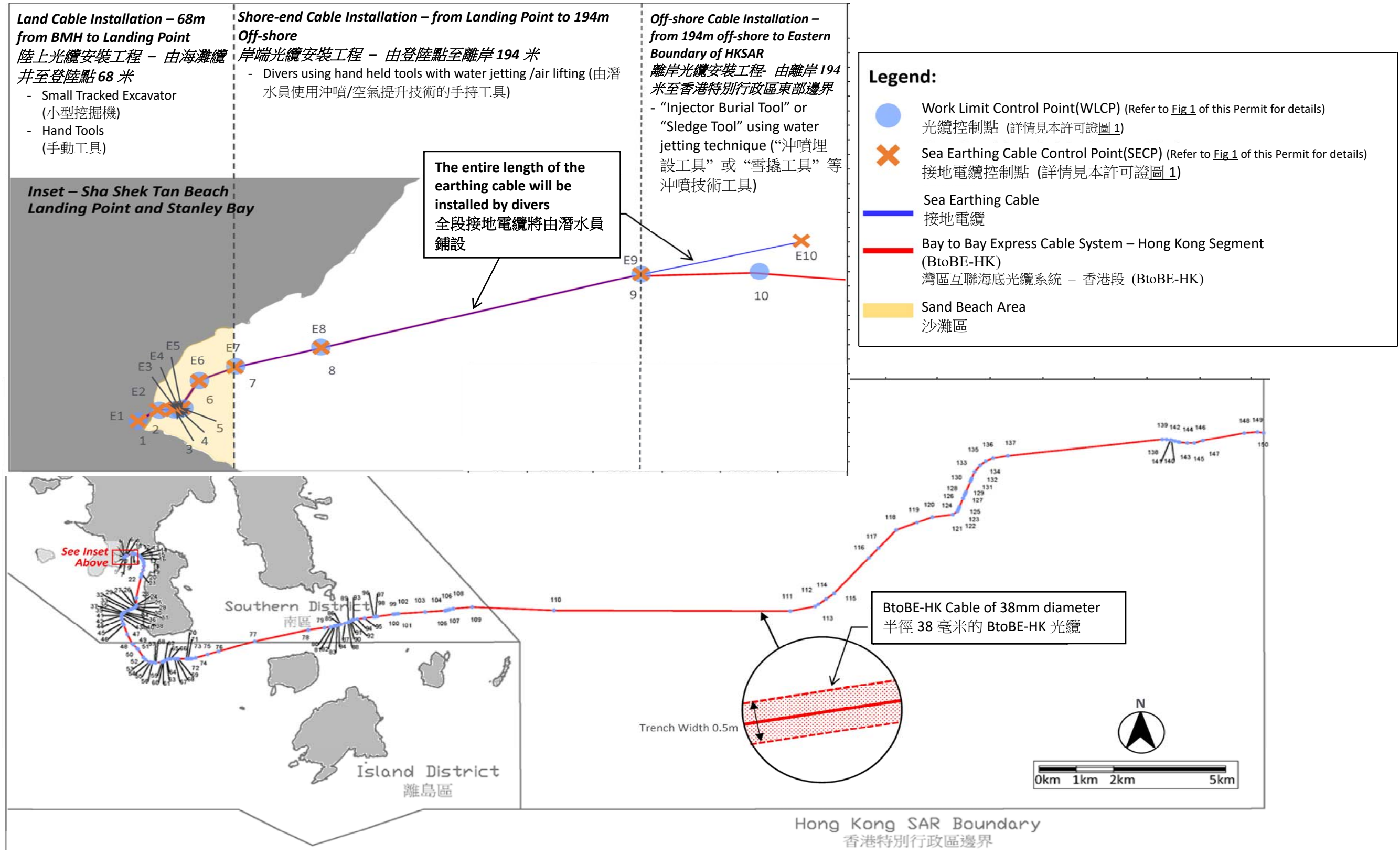
Project Title 工程項目名稱 Bay to Bay Express Cable System - Hong Kong Segment (BtoBE-HK) - Chung Hom Kok 灣區互聯海底光纜系統 - 香港段(BtoBE-HK) - 春坎角 Figure 4: 圖 4 Installation Method of the Cable 光纜系統的安裝方法
