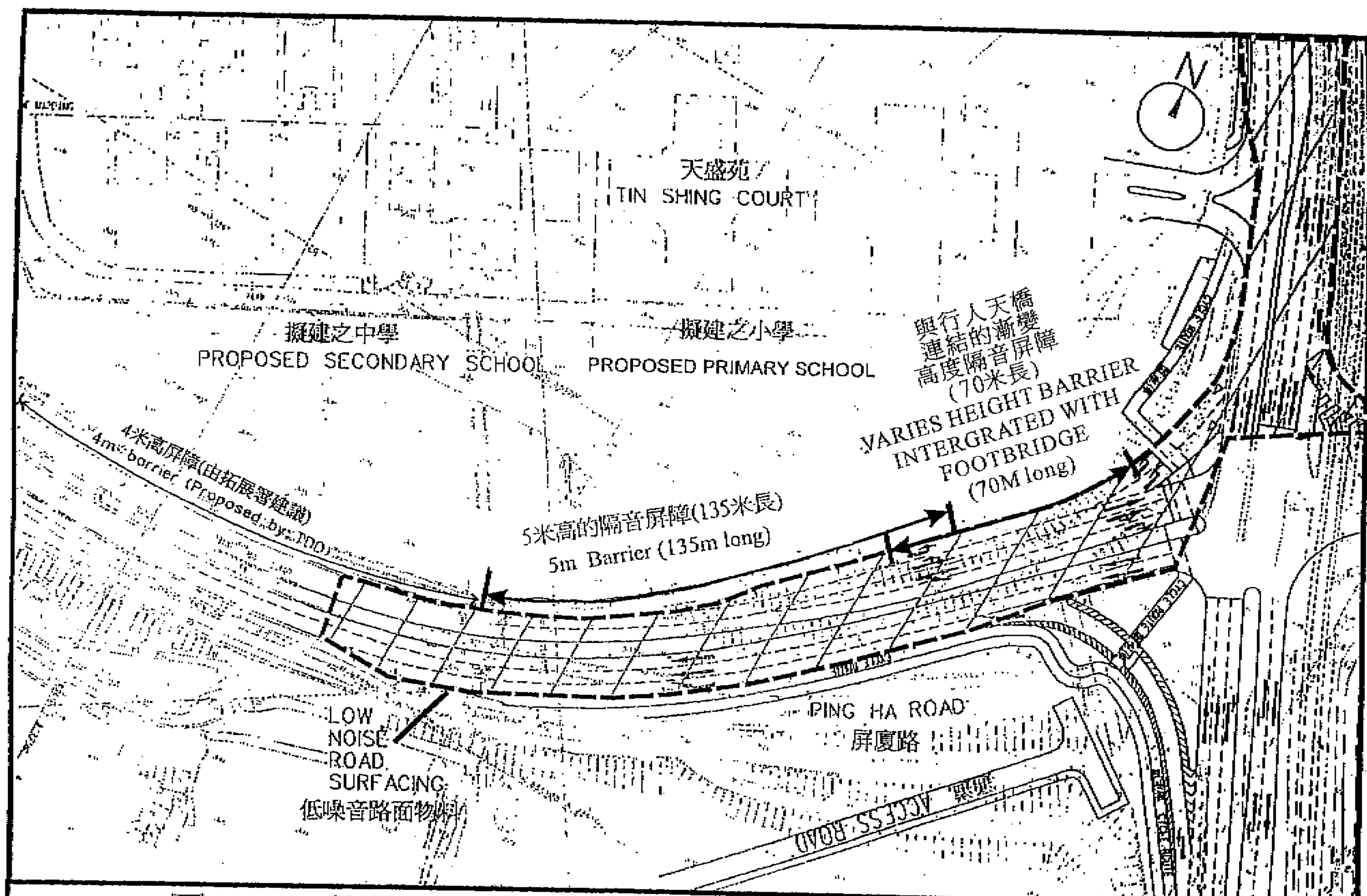
圖5.1 - 位於天水圍屏廈路的道路交通噪音直接緩減設施 FIGURE 5.1 - Direct Road Traffic Noise Mitigation Measures on Ping Ha Road, Tin Shui Wai
