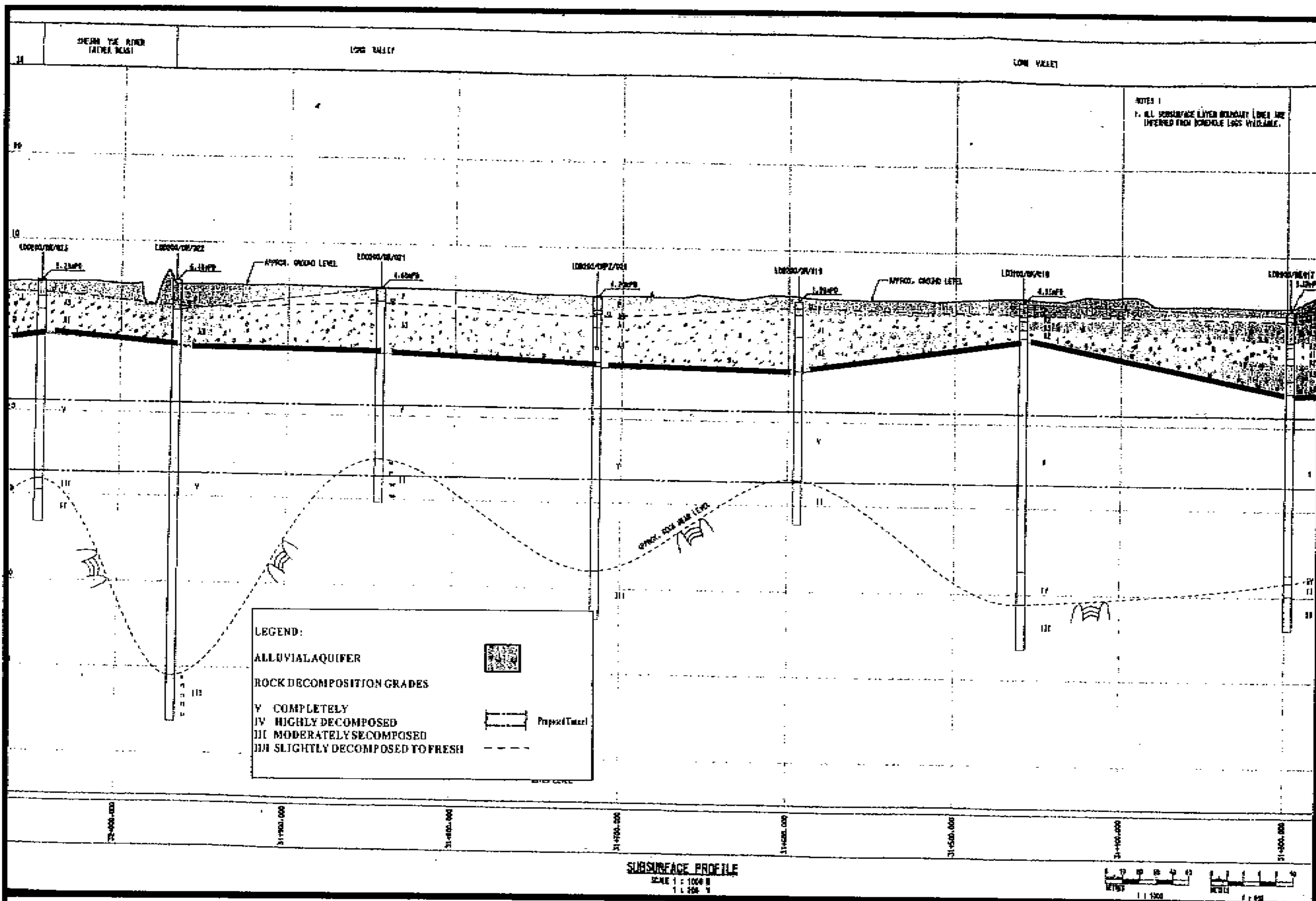
Figure 5 - Sheung Shui to Lok Ma Chau Spur Line (上水至落馬洲支線) 圖五 - 條例3.9所指貫穿塹原之隧道垂直側面圖 (Reproduced from Figure I of Appendix A3.1 of the EIA Report (Register No.: ABIAR-052/2002) 摘自至環評報告附件A3.1圖 - (登記冊編號: ABIAR - 052/2002)
