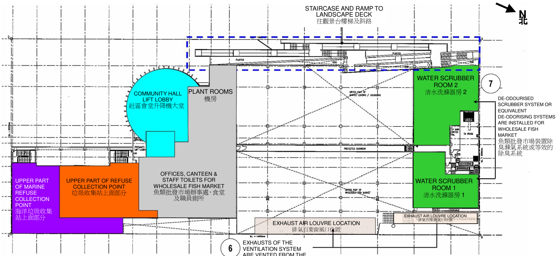
MEZZANINE FLOOR PLAN 閣樓平面圖
