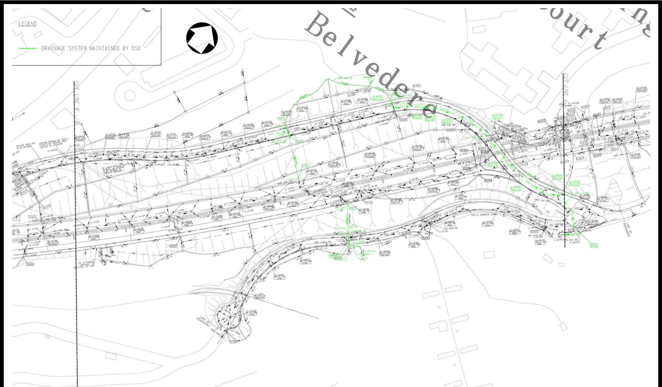
Project Title: Trunk Road T7 in Ma On Shan Figure D4: Drainage Plan (Drainage Services Department) (Sheet 3 of 8) [Extracted from the Figure D4 of FEP Application (Application No.: FEP-131/2012)]
