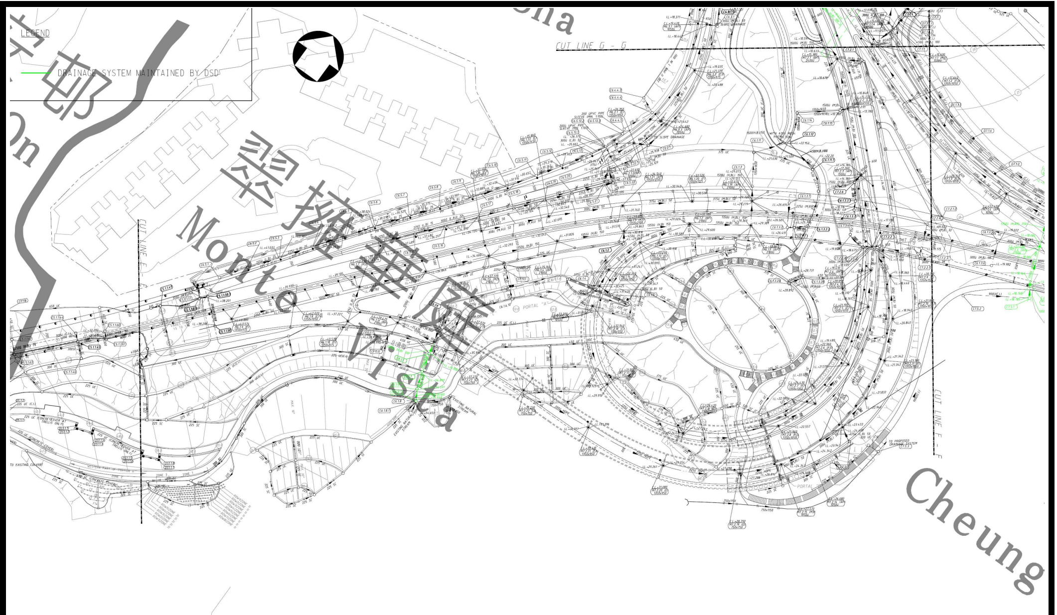
Project Title: Trunk Road T7 in Ma On Shan Figure D7: Drainage Plan (Drainage Services Department) (Sheet 6 of 8) [Extracted from the Figure D7 of FEP Application (Application No.: FEP-131/2012)]
