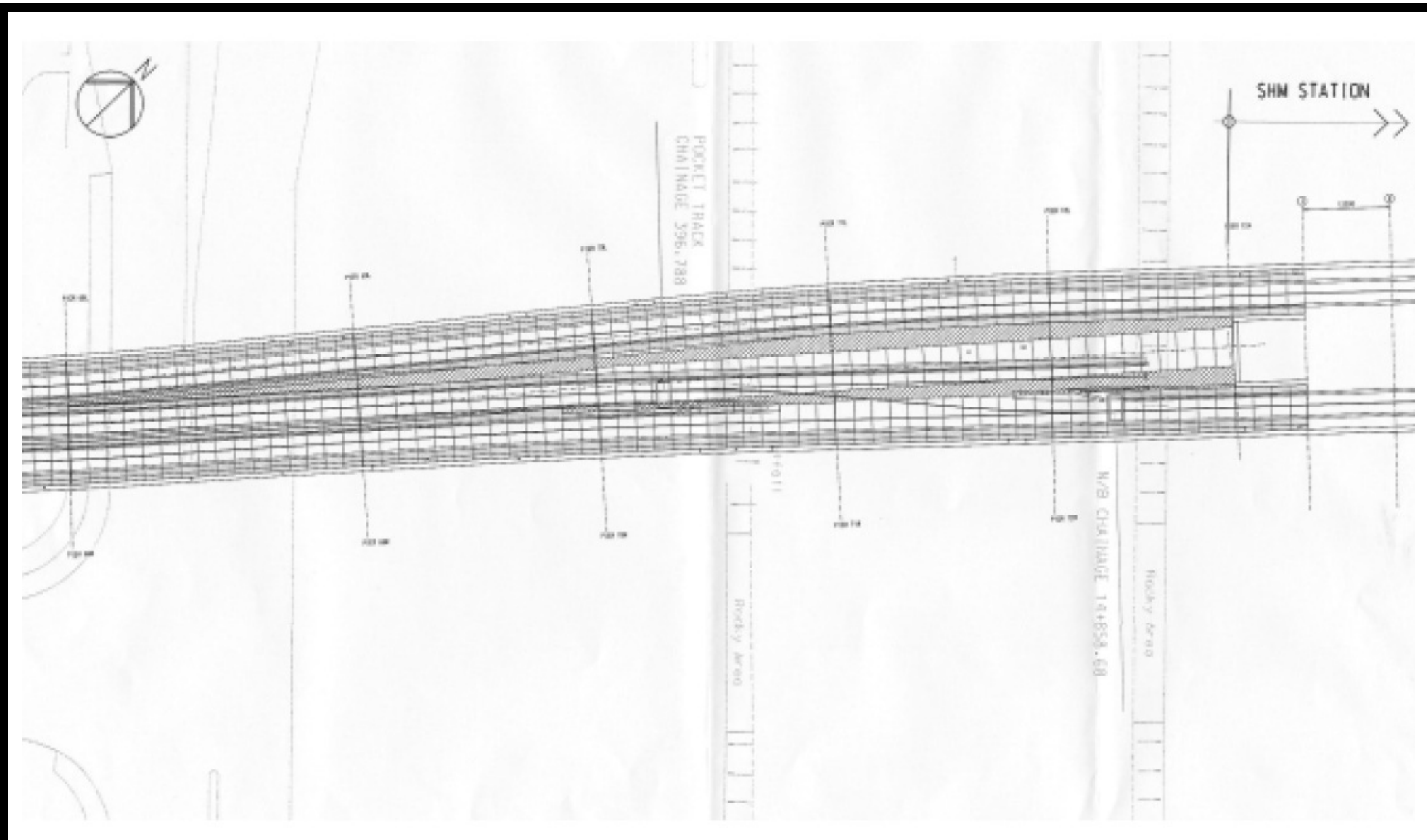
Project Title: East Rail Extensions - Tai Wai to Ma On Shan Figure 13: Point machine locations between City One Station and Shek Mun Station [Extracted from the Figure 13 of FEP Application (Application No.: FEP-132/2012)]
