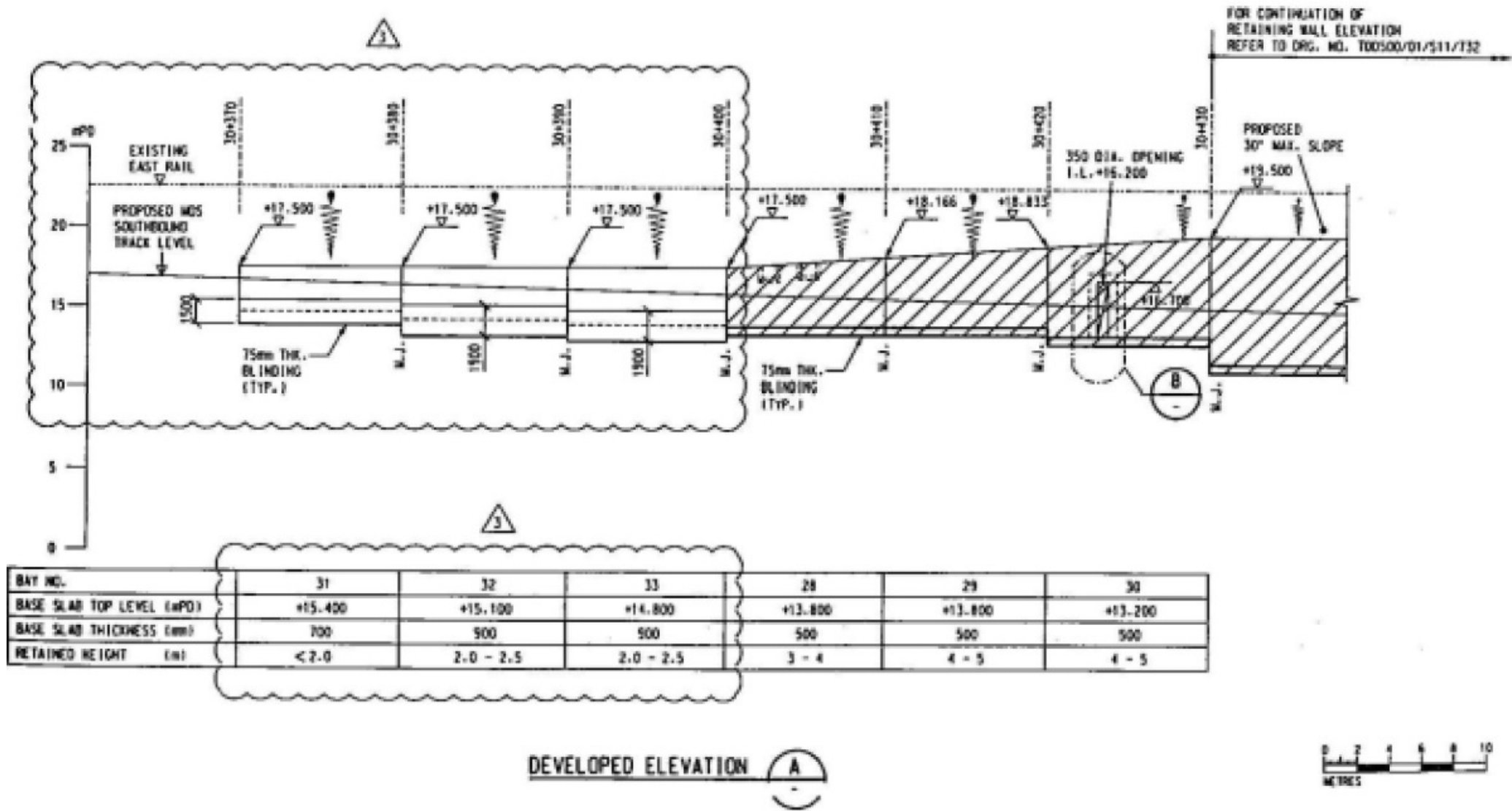
Project Title: East Rail Extensions - Tai Wai to Ma On Shan Figure 18: Retaining Wall RW3A [Extracted from the Figure 18 of FEP Application (Application No.: FEP-132/2012)]
