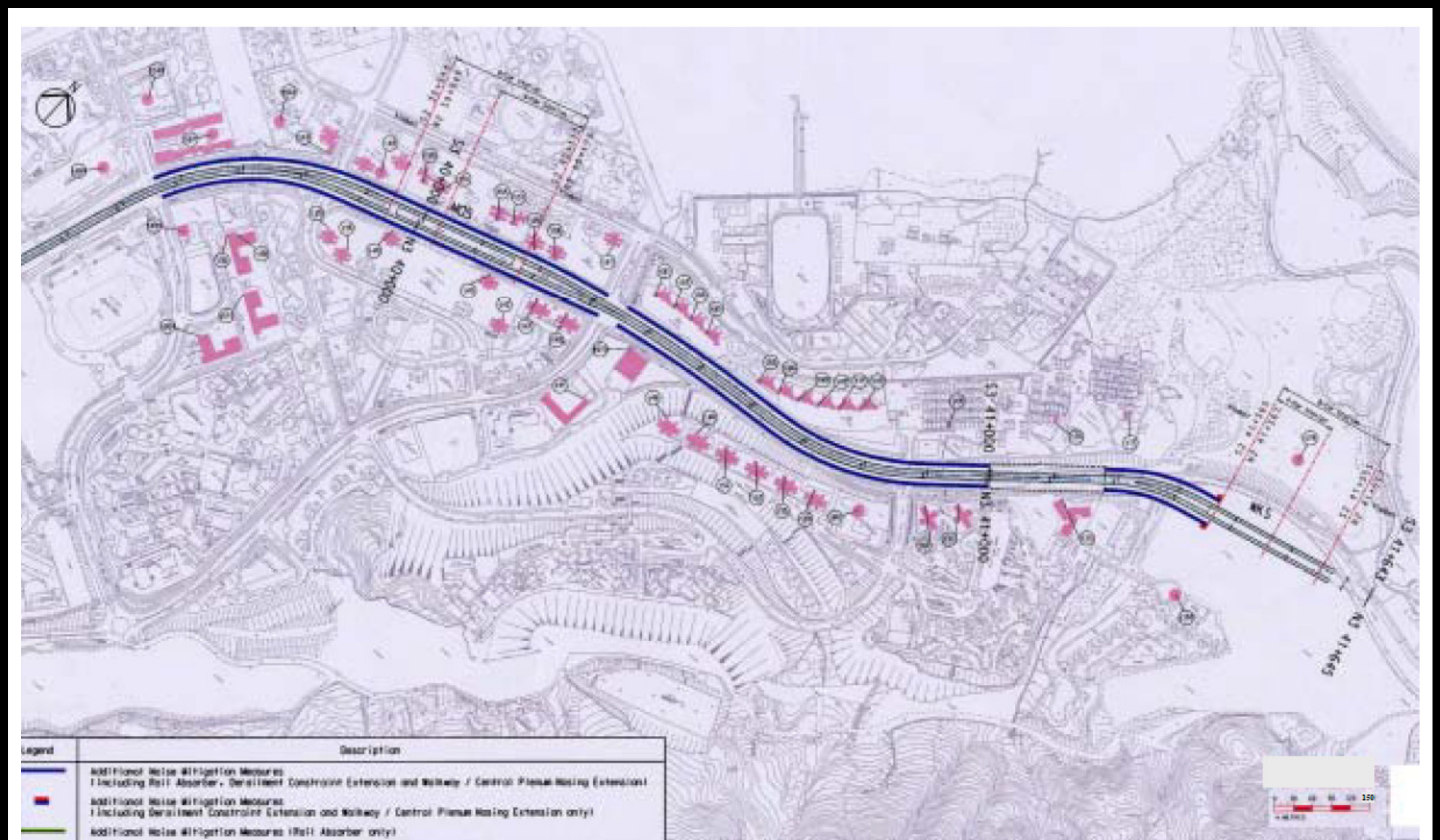
Project Title: East Rail Extensions - Tai Wai to Ma On Shan Figure 25: Locations of Additional Noise Mitigation Measures [Extracted from the Figure 1 of FEP Application (Application No.: FEP-132/2012)]
