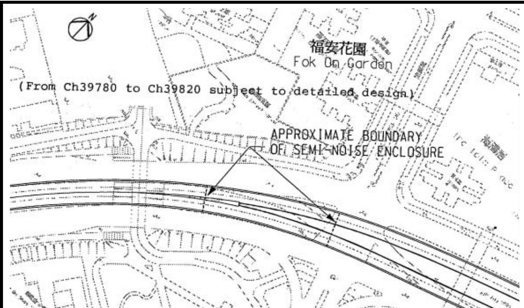
Project Title: East Rail Extensions - Tai Wai to Ma On Shan Figure 30: Noise Enclosure Fronting Fok On Garden [Extracted from the Figure 30 of FEP Application (Application No.: FEP-132/2012)]
