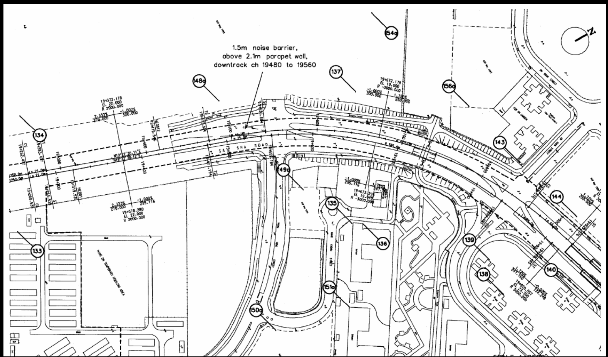
Project Title: East Rail Extensions - Tai Wai to Ma On Shan Figure 9: Noise Barriers and Enclosures [Extracted from the Figure 9 of FEP Application (Application No.: FEP-132/2012)]
