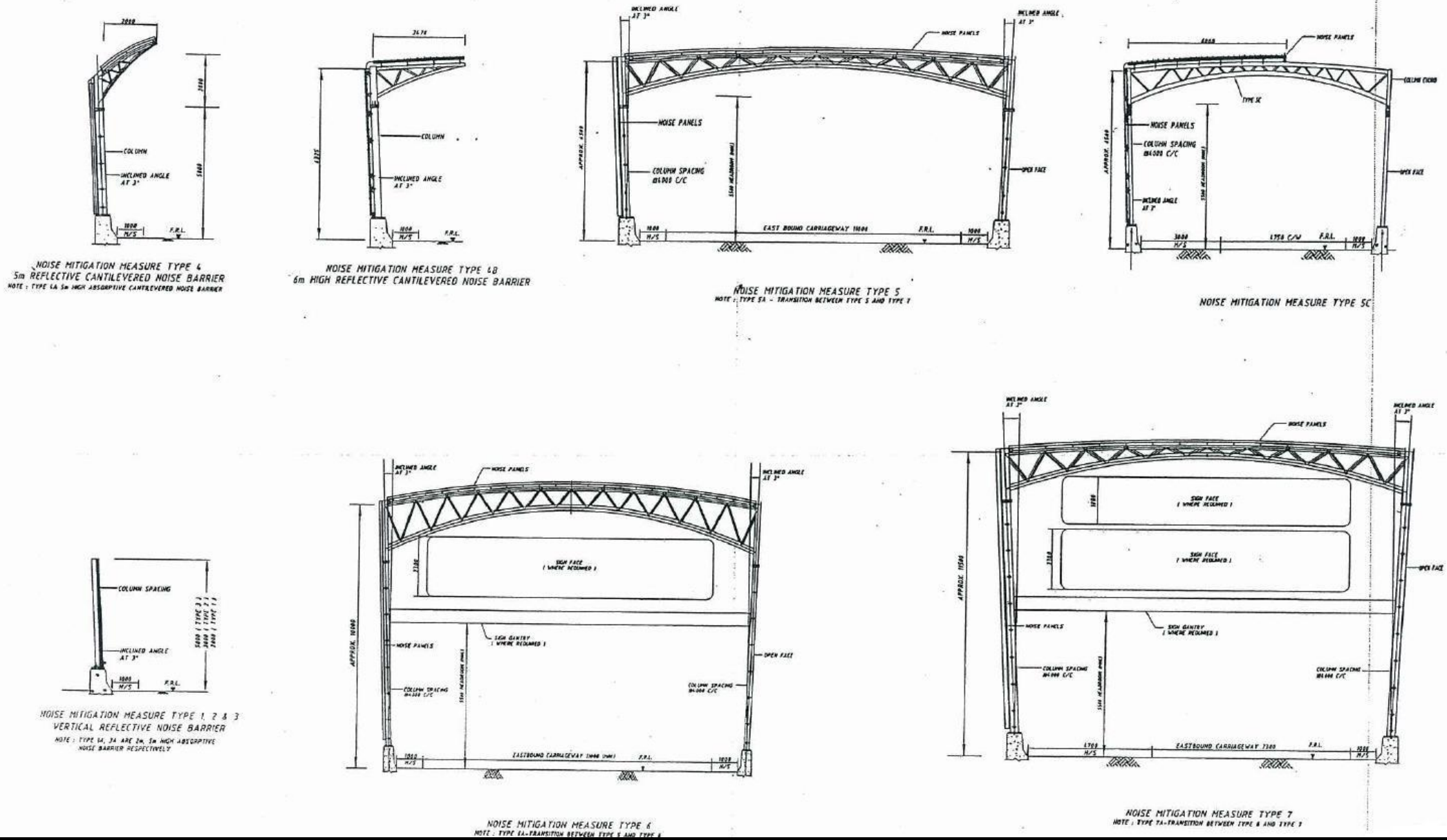
Project Title: Trunk Road T7 in Ma On Shan Figure 3: Noise Mitigation Measures Cross Sections
