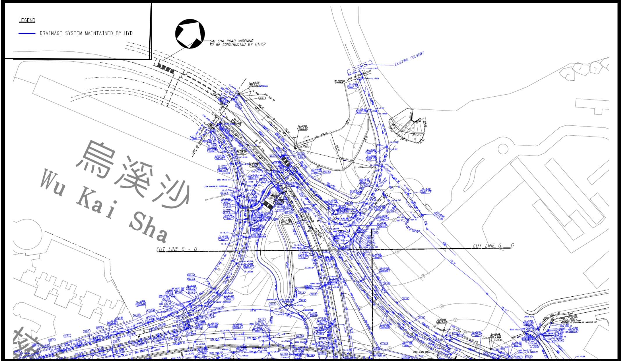
Project Title: Trunk Road T7 in Ma On Shan Figure H21: Drainage Plan of Highways Department (HYD) (Sheet 8 of 8)
