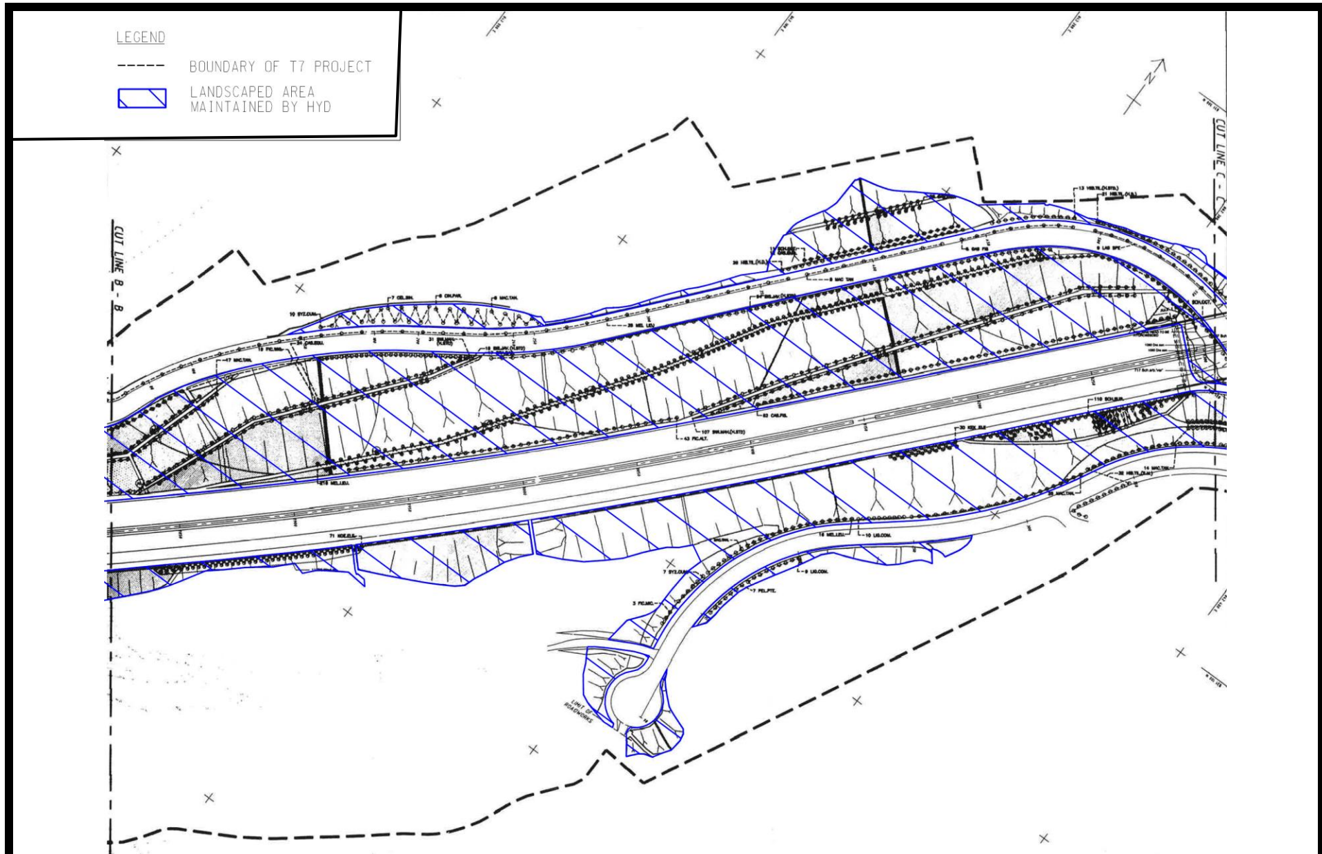
Project Title: Trunk Road T7 in Ma On Shan Figure H5: Landscape Maintenance Plan of Highways Department (HYD) (Sheet 3 of 10)
