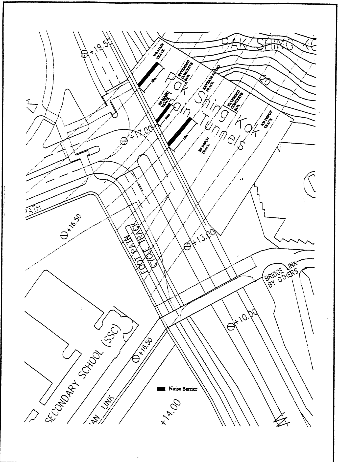
FIGURE F - Proposed Location and Length of the Noise Barriers along the EB Main Track, WB Main Track and the Reverse Siding Track
