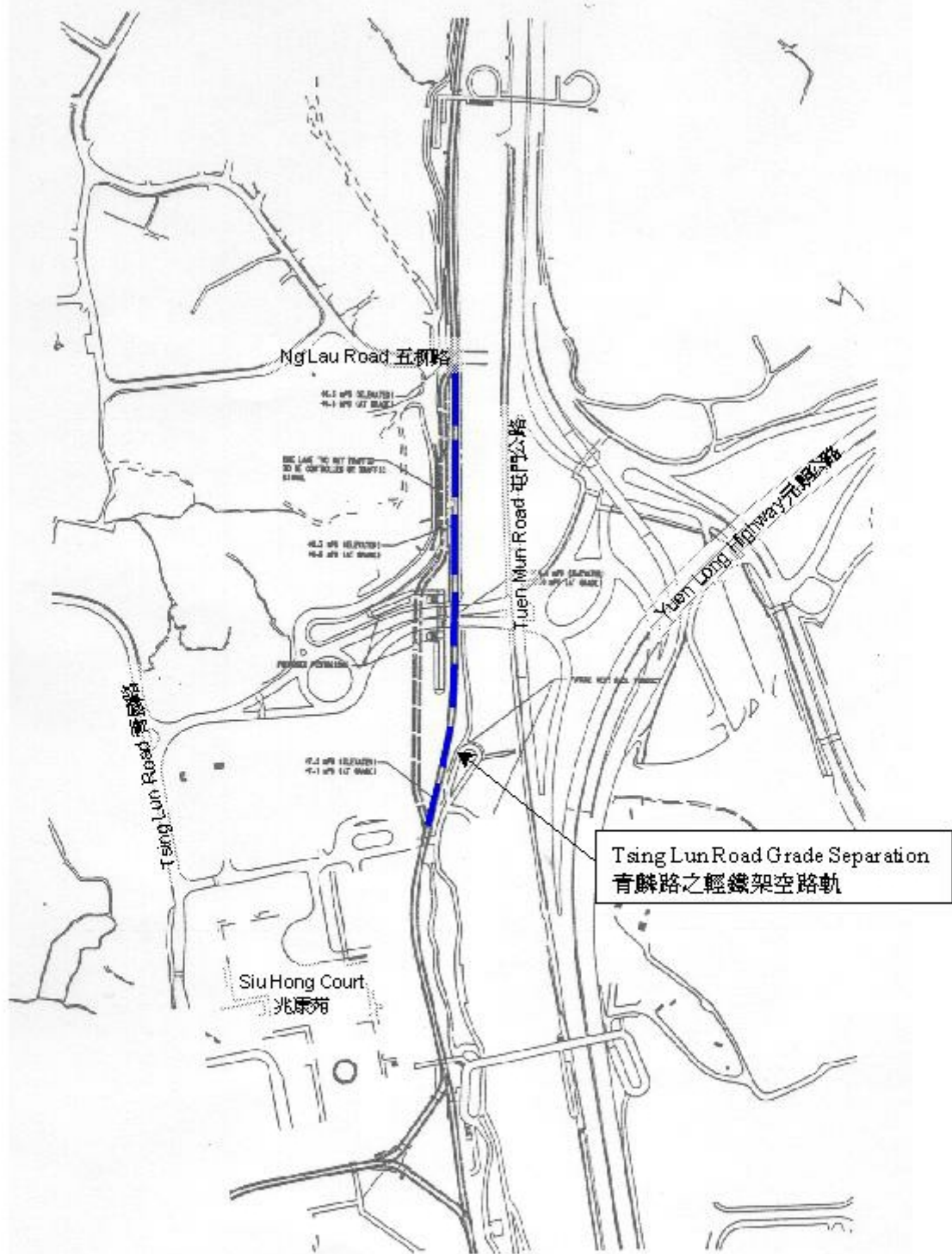
Figure 3 Location Plan 地點圖 附圖三 Tsing Lun Road Grade Separation 青麟路之輕鐵架空路軌
