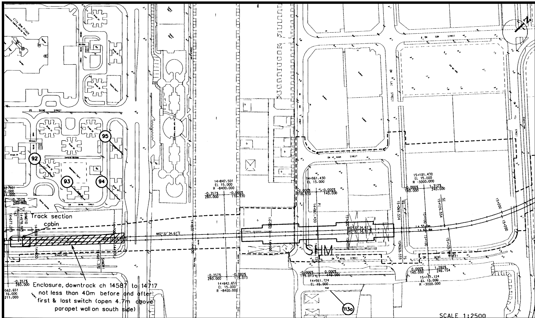
Figure 4 Noise Barriers and Enclosures (Extracted from Technical Annex F1 of the EIA Report)
