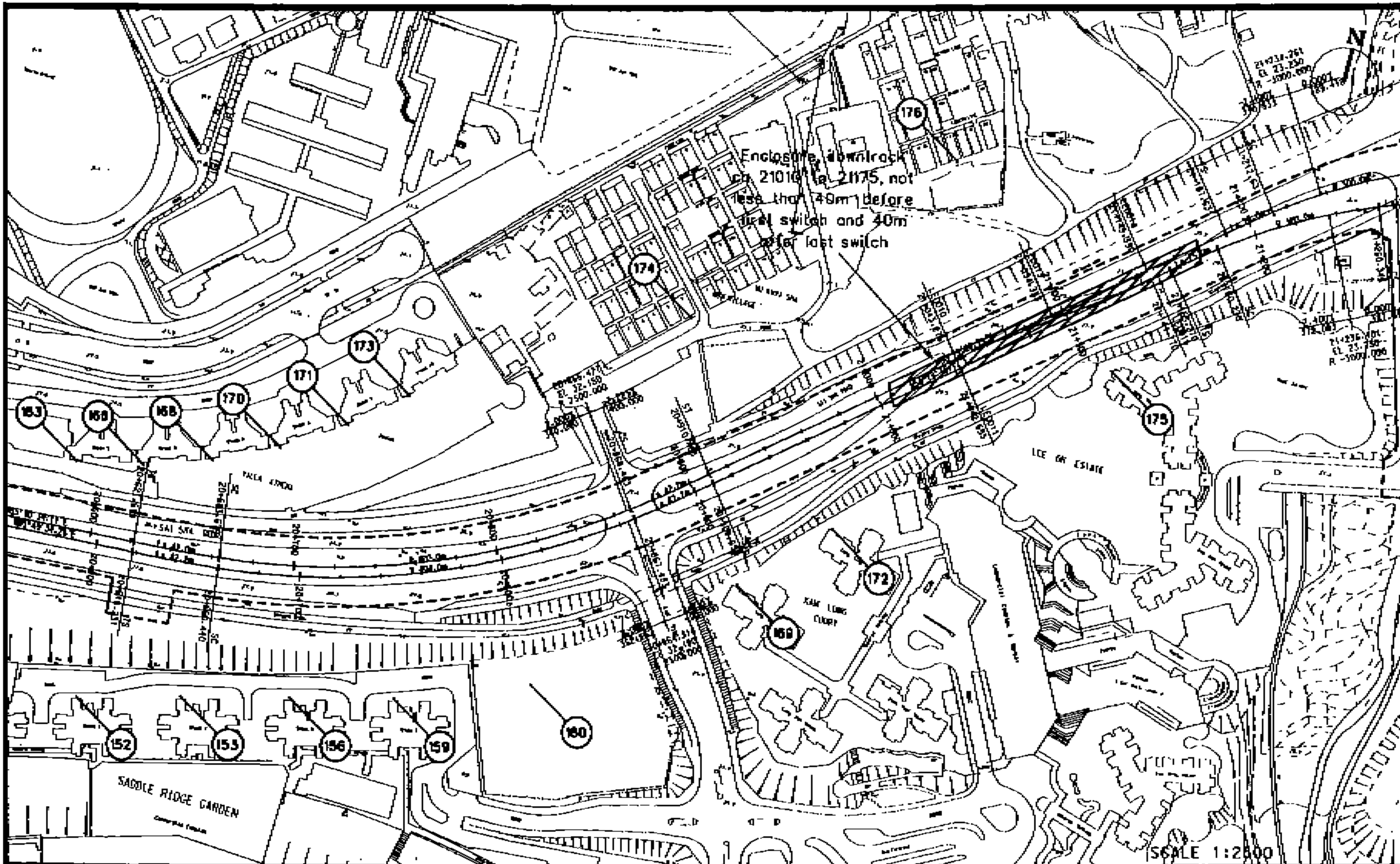
Figure 10 Noise Barriers and Enclosures (Extracted from Technical Annex F1 of the EIA Report)
