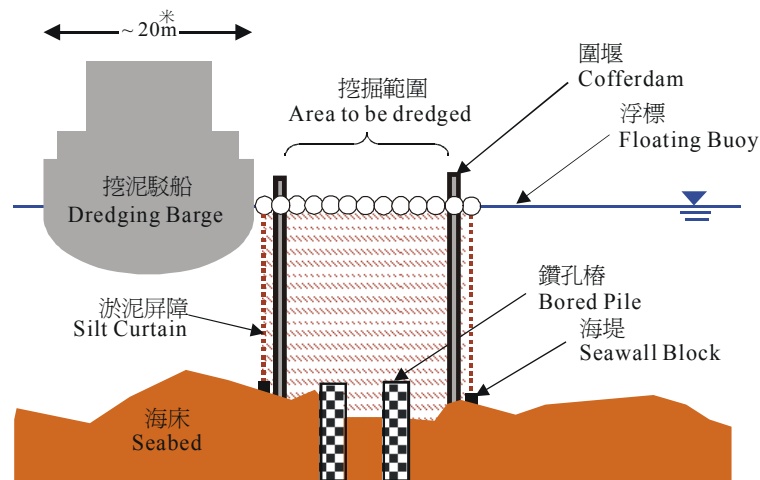
淤泥屏障布置的橫切面 (c) Cross-section of Silt Curtain Arrangement
