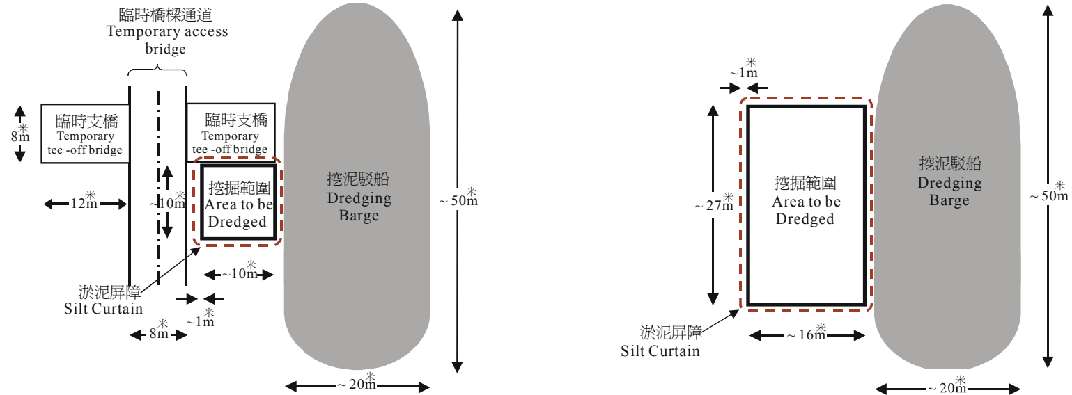
典型跨部分橋墩地點的淤泥屏障布置 (a) Silt Curtain Arrangement for Typical Span Pier Site
