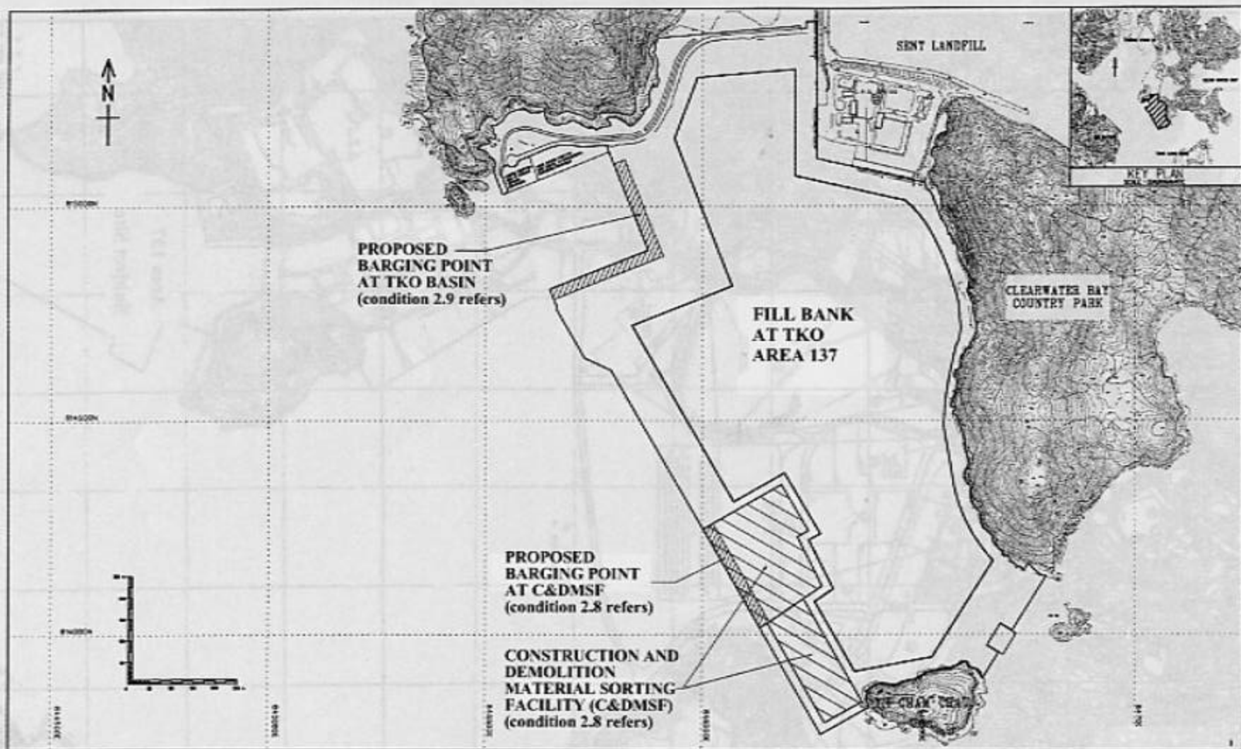
Figure 2 : Locations of the Proposed Barging Points
