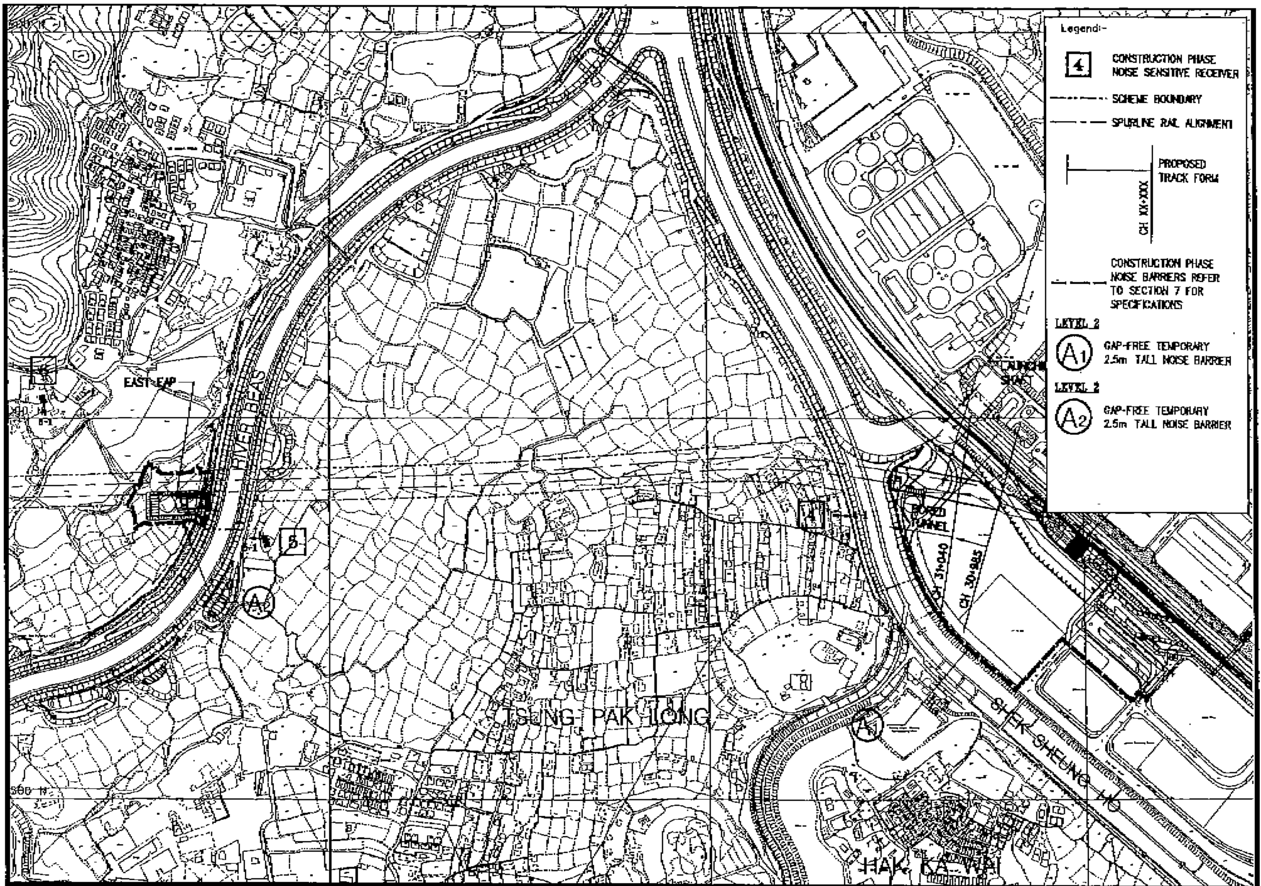
Sheung Shui to Lok Ma Chau Spur Line (上水至落馬州支線) Figure 7b - Locations of Construction Phase Noise Barriers as described in Condition 3.17 of the Permit 圖七乙 - 條例3.17所指消除建築工程噪音之隔音屏障位置 Reproduced from Drawing No. 7.1 (Sheet 2 of 5) (Volume 5 of 5) of the EIA Report (Register number AEIAR-052/2002) 摘自環評報告第五冊圖7.1(第二張)(登記冊編號AEIAR-052/2002)
