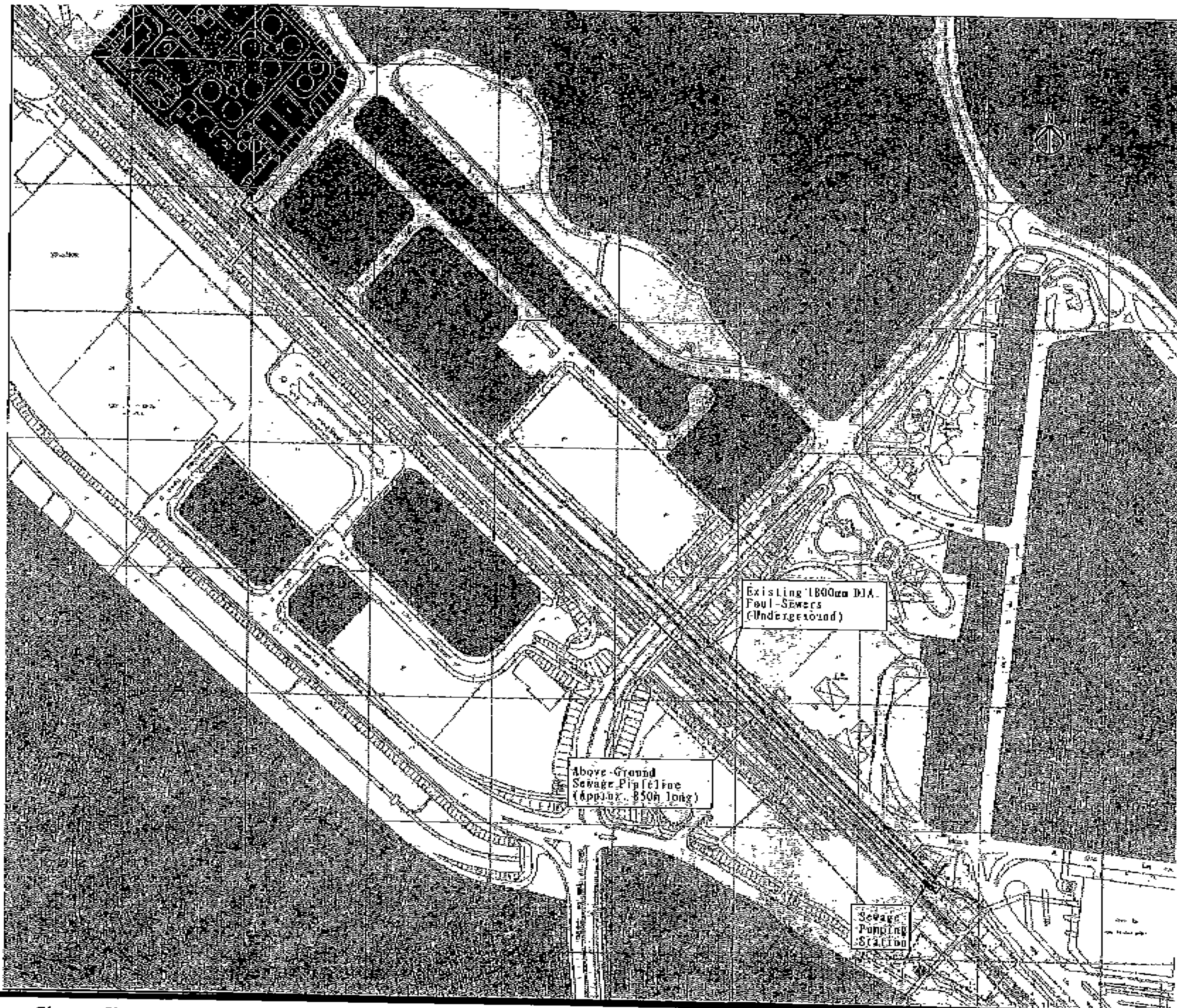
Figure 9 - Sheung Shui to Lok Ma Chau Spur Line (上水至落馬州支線) 圖九 - 污水渠緊急旁道系統平面圖 Reproduced from Drawing No. LDB-201/000/73/C84/574 as submitted in application number VEP-102/2003 摘自申請書編號 VEP-102/2003 圖 LDB-201/000/73/C84/574
