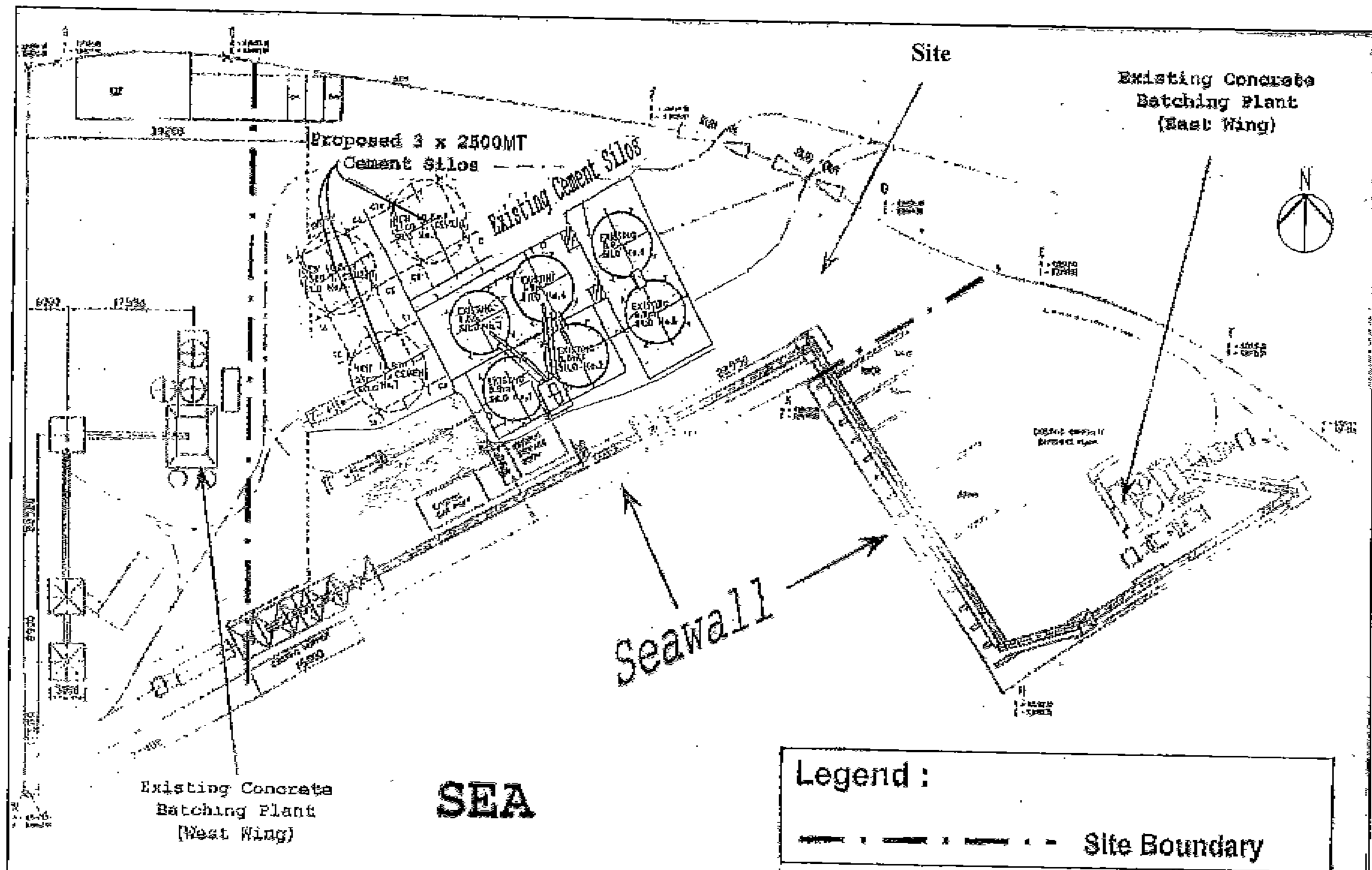
Figure 2 Site Layout Plan for Cement Depot (Extracted from Application VEP-103/2003)
