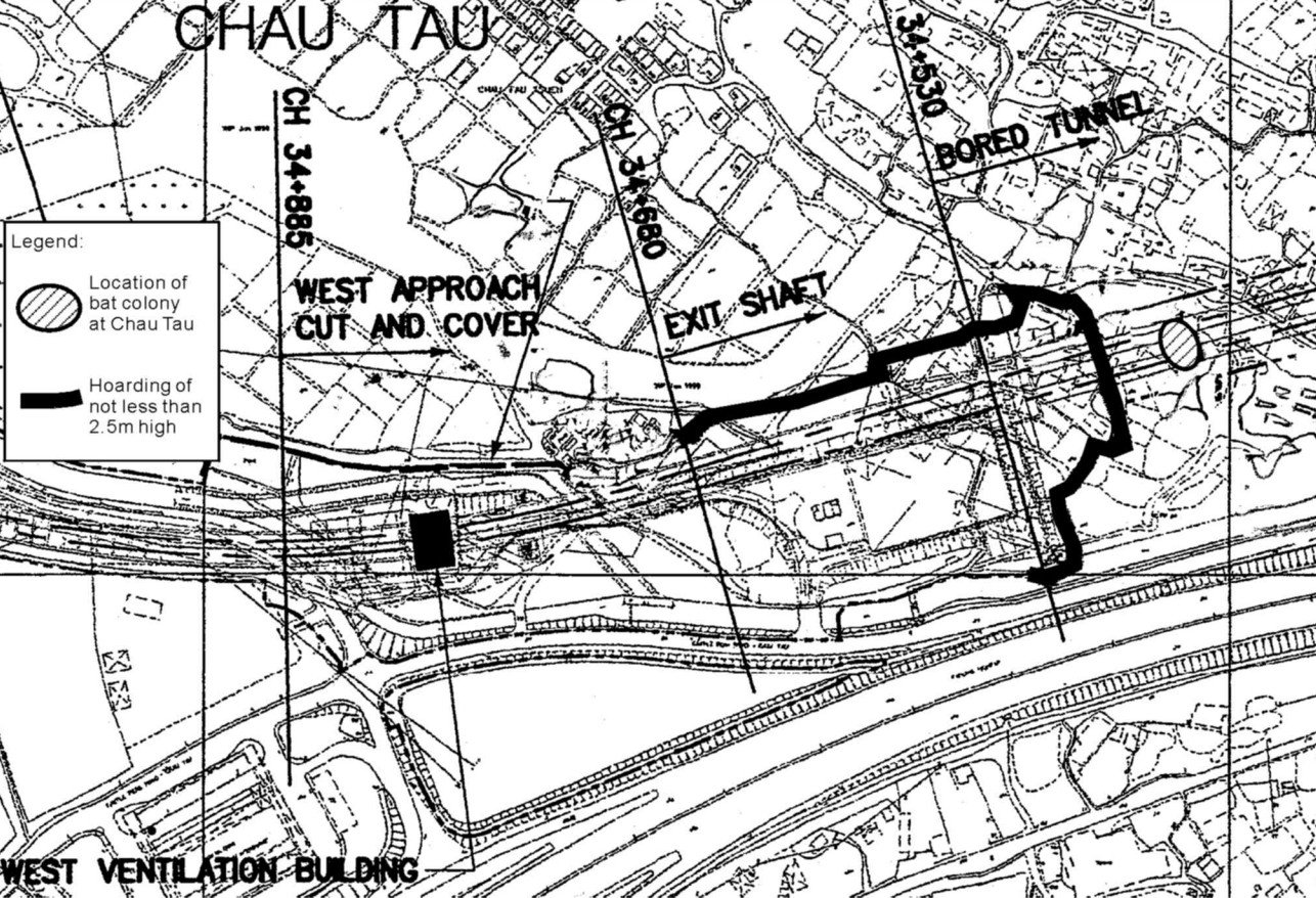
Figure 6 - Sheung Shui to Lok Ma Chau Spur Line (上水至落馬州支線) Locations of the bat colony at Chau Tau and Site Hoarding to be erected as described in Condition 3.14 of the Permit 圖六- 在洲頭的蝙蝠群居地和條例3.14所指的地盤圍街板位置
