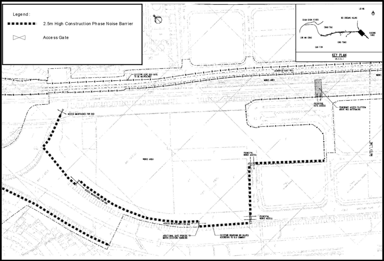
Figure 7a - Locations of Construction Phase Noise Barriers as described in Condition 3.17 of the Permit 圖七甲 - 條例3.17所指消除建築工程噪音之隔音屏障位置
