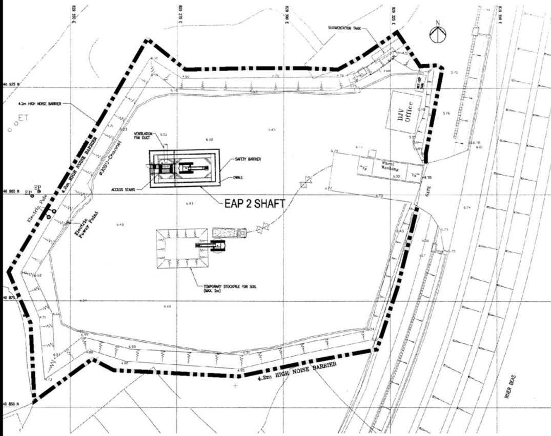
Figure 7b - 圖七乙 - Sheung Shui to Lok Ma Chau Spur Line (上水至落馬州支線) Locations of Construction Phase Noise Barriers as described in Condition 3.17 of the Permit 條例3.17所指消除建築工程噪音之隔音屏障位置 Reproduced from Drawing No. LDB-201/001/92/C83/003 as submitted in Application No. VEP-130/2004 摘自申請書編號 VEP-130/2004 圖 LDB-201/001/92/C83/003
