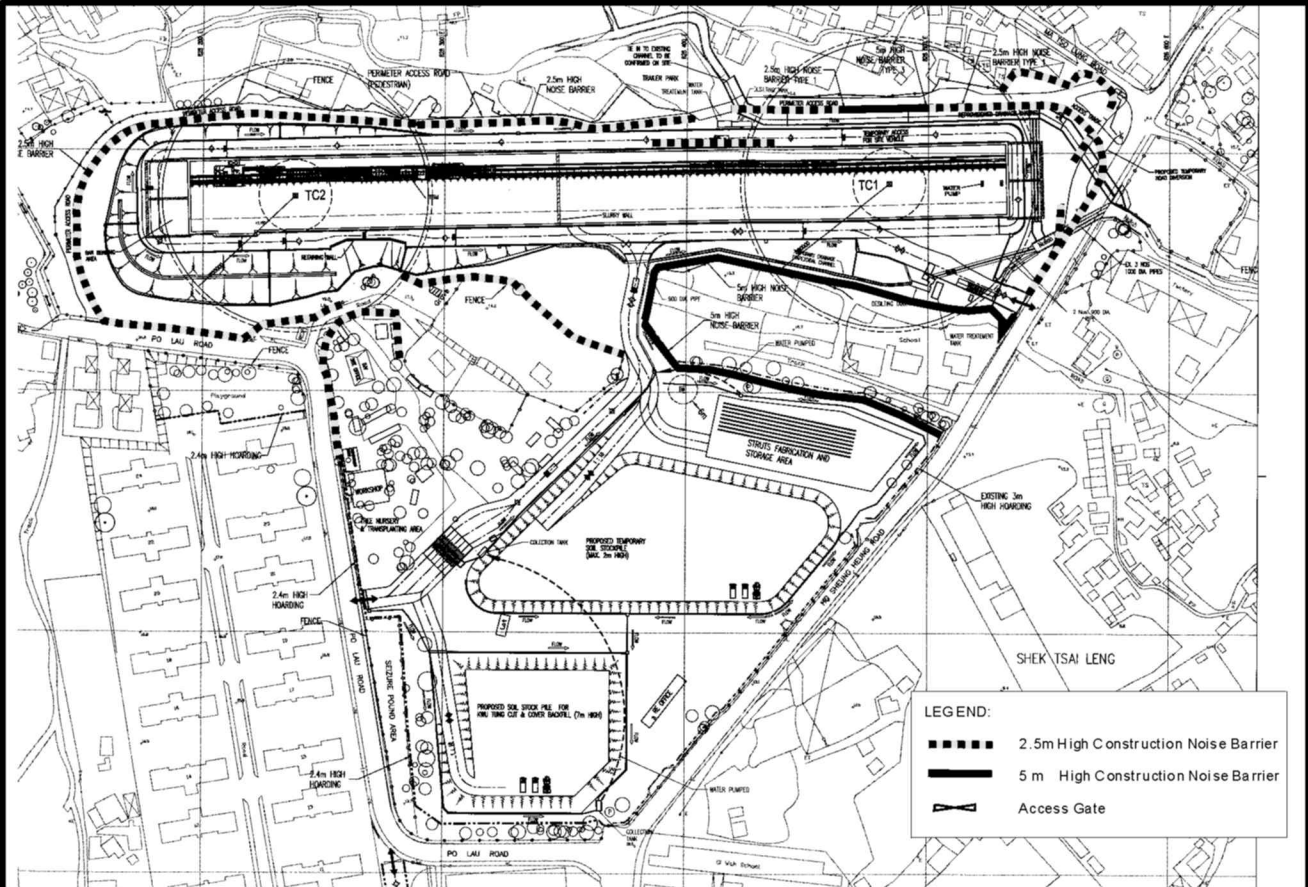
Figure 7c - Locations of Construction Noise Barriers as described in Condition 3.17 of the Permit 圖七丙 - 條例3.17所指消除建築工程噪音之隔音屏障位置 Reproduced from Drawing No. LDB-201/000/18/C84/800 as submitted in Application No. VEP-130/2004 摘自申請書編號 VEP-130/2004 圖 LDB-201/000/18/C84/800
