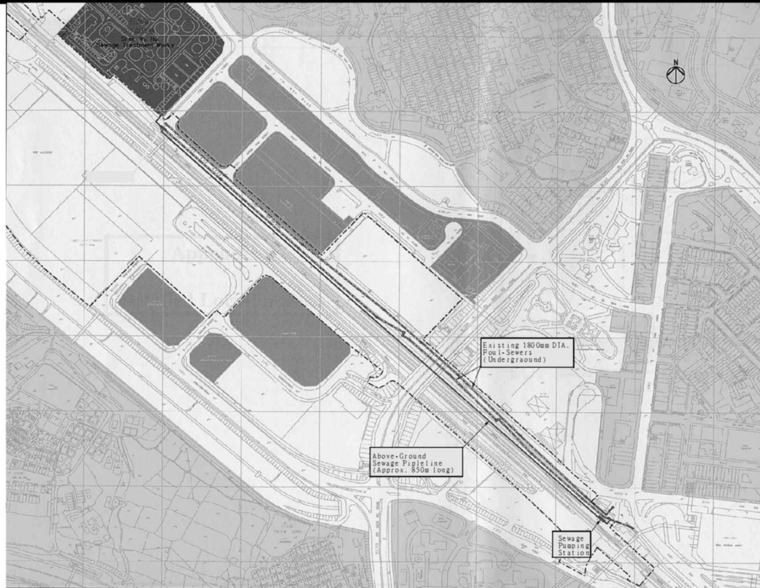
Figure 9 - Sheung Shui to Lok Ma Chau Spur Line (上水至落馬州支線) 圖九 - 污水渠應急旁道系統平面圖 Reproduced from Drawing No. LDB-201/000/73/C84/574 as submitted in application number VEP-102/2003 擴自申請書編號VEP-102/2003 圖LDB-201/000/73/C84/574
