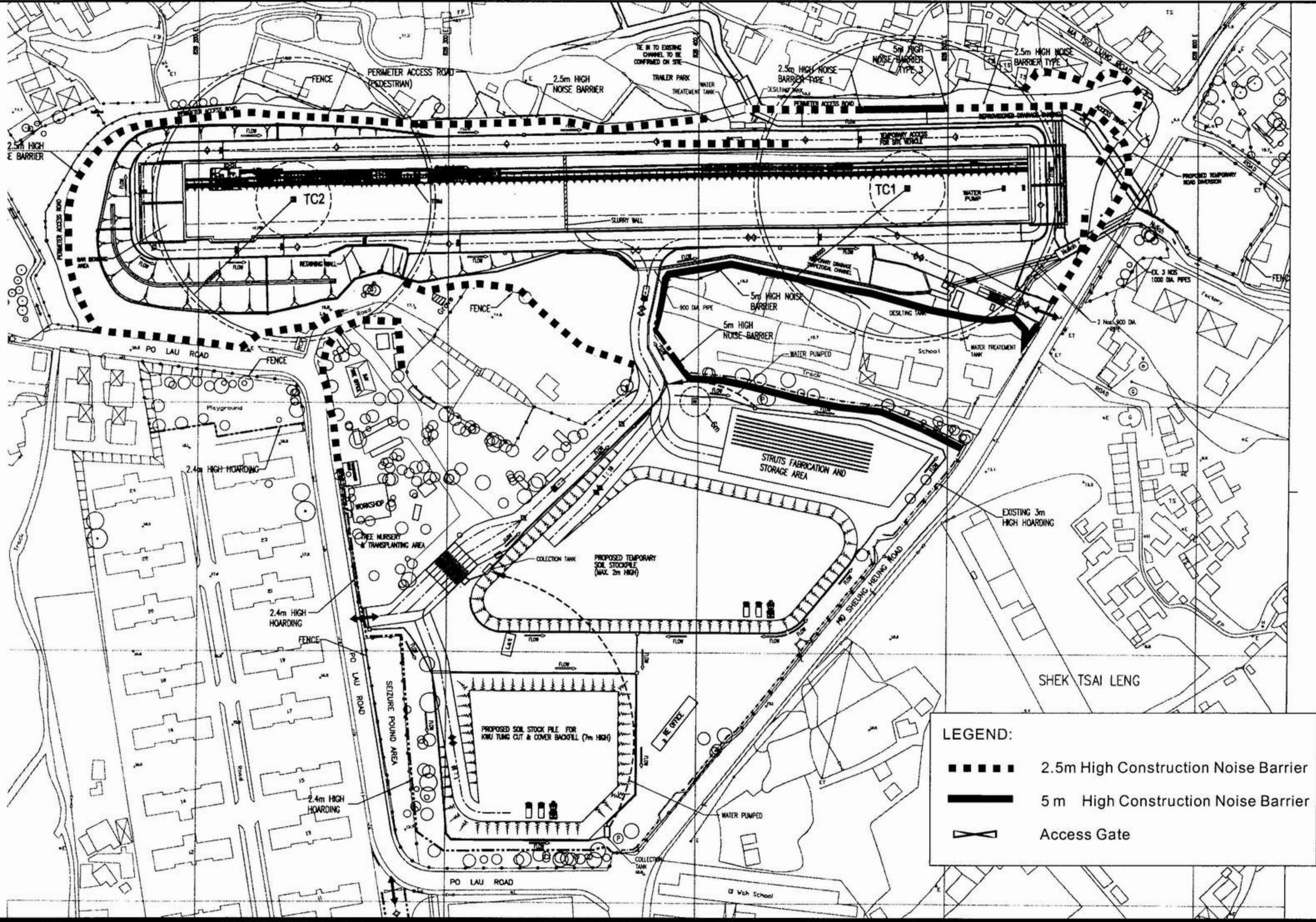
Figure 7c - Locations of Construction Noise Barriers as described in Condition 3.17 of the Permit 圖七丙 - 條例3.17所指消除建築工程噪音之隔音屏障位置 Reproduced from Drawing No. LDB-201/000/18/C84/800 as submitted in Application No. VEP-130/2004 摘自申請書編號VEP-130/2004圖LDB-201/000/18/C84/800
