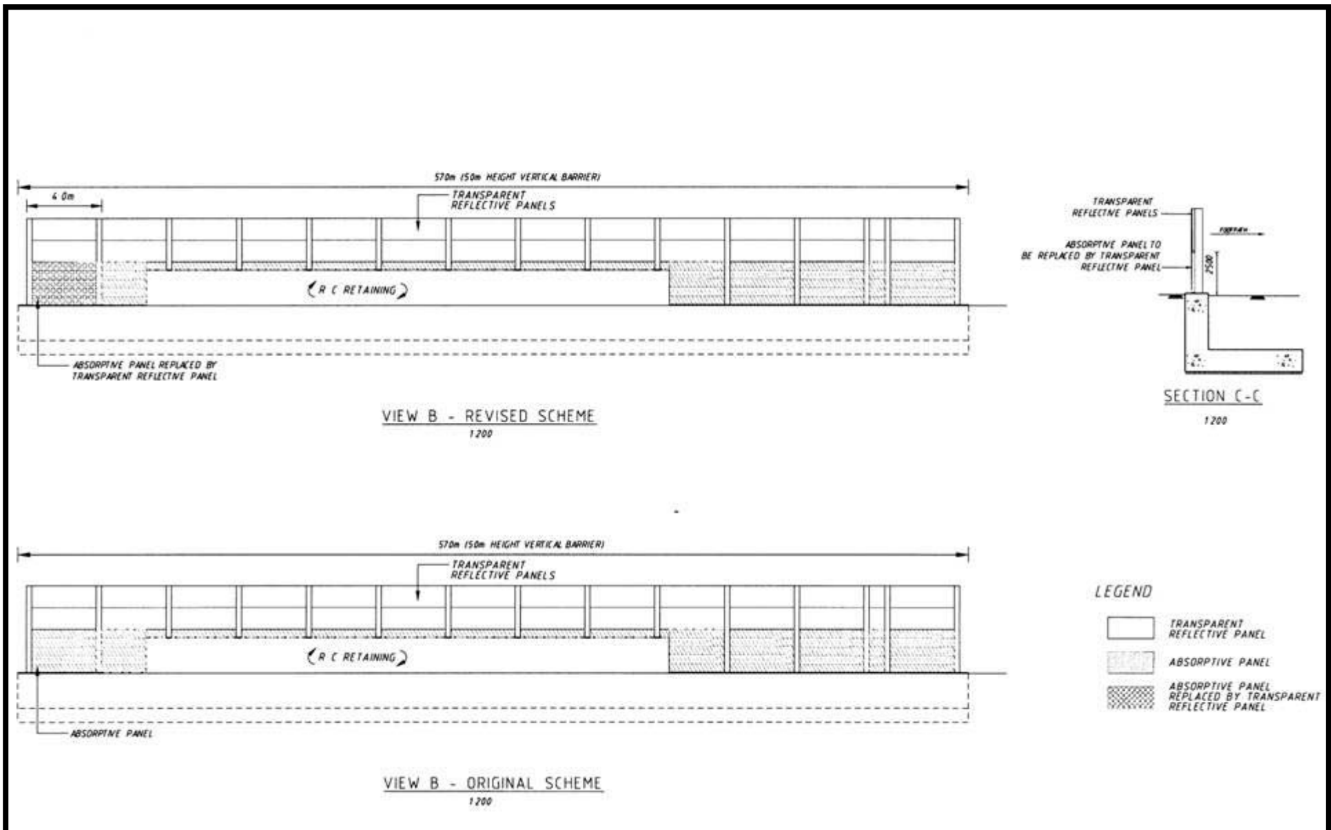
Sha Tin New Town – Stage II, Road T3 and Associated Roadworks Figure 11 – Extent of noise barrier segment no. 48 where absorptive panels as originally provided to a height of 2.5m above the road level are replaced by transparent reflective panels (Extracted from the Application VEP-169/2005)
