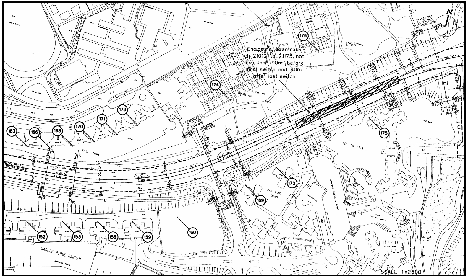
Figure 10 Noise Barriers and Enclosures (Extracted from Technical Annex F1 of the EIA Report)
