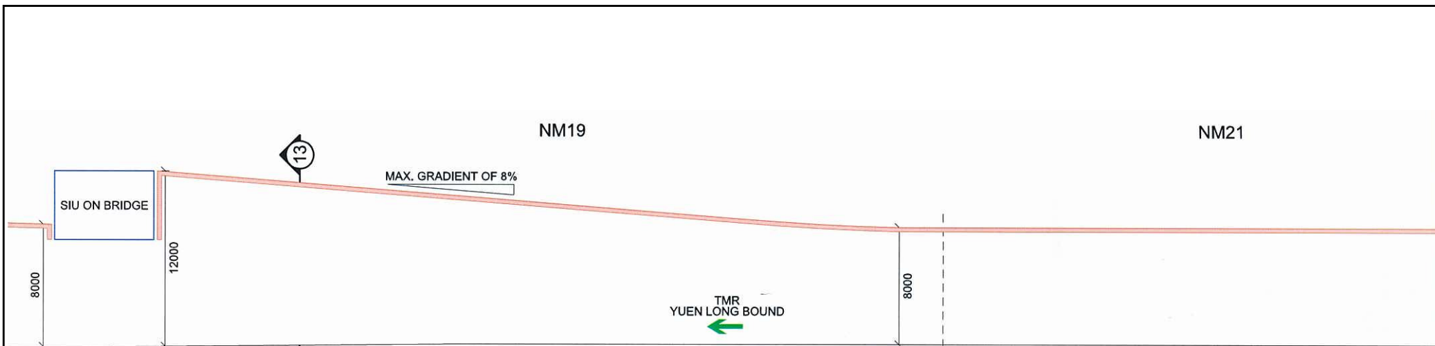
LONGITUDINAL SECTION ALONG TMR YUEN LONG BOUND BETWEEN NM19 AND NM21 (N.T.S)
