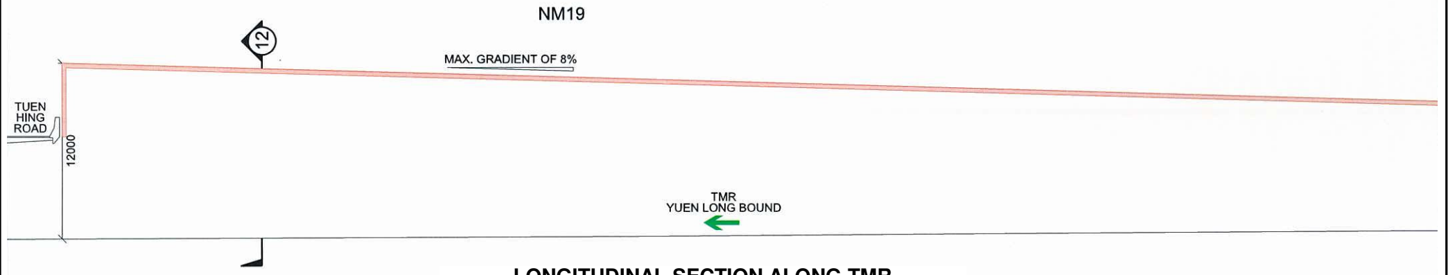
LONGITUDINAL SECTION ALONG TMR YUEN LONG BOUND at NM19 (N.T.S)
