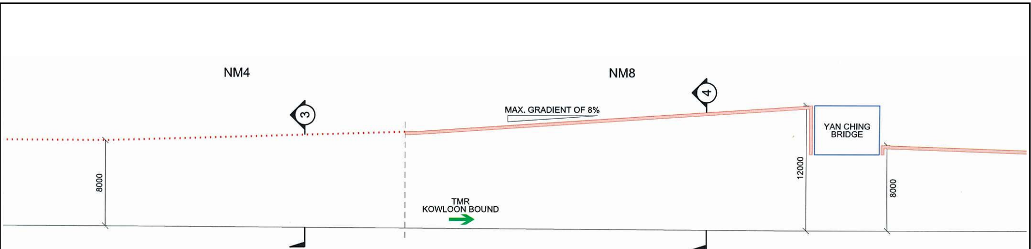
LONGITUDINAL SECTION ALONG TMR KOWLOON BOUND BETWEEN NM4 AND NM8 (N.T.S.)
