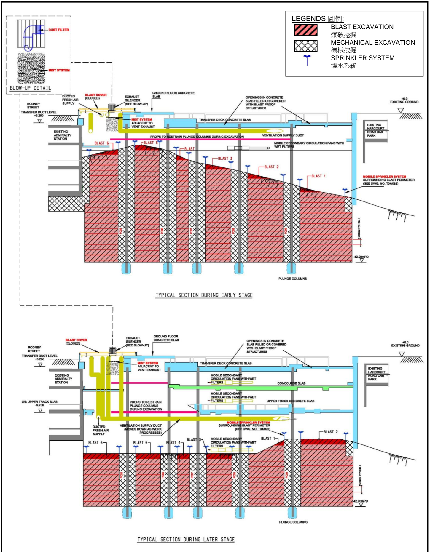
Figure 19: Location of Sprinkler and Ventilation System
