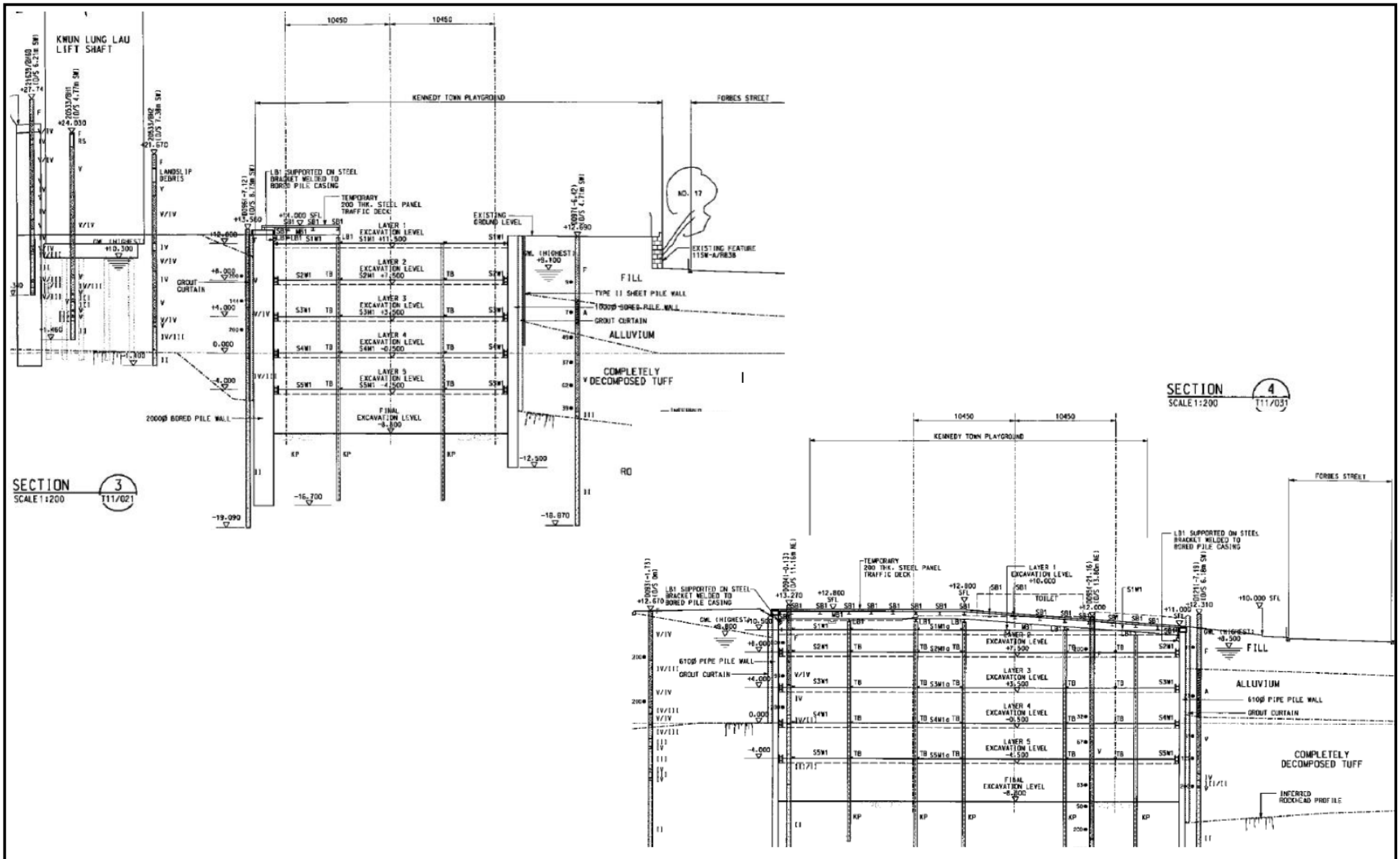
Figure 12: Sections of Decking at Works Area C 圖 12: 施工區丙的大概鋪蓋切面圖
