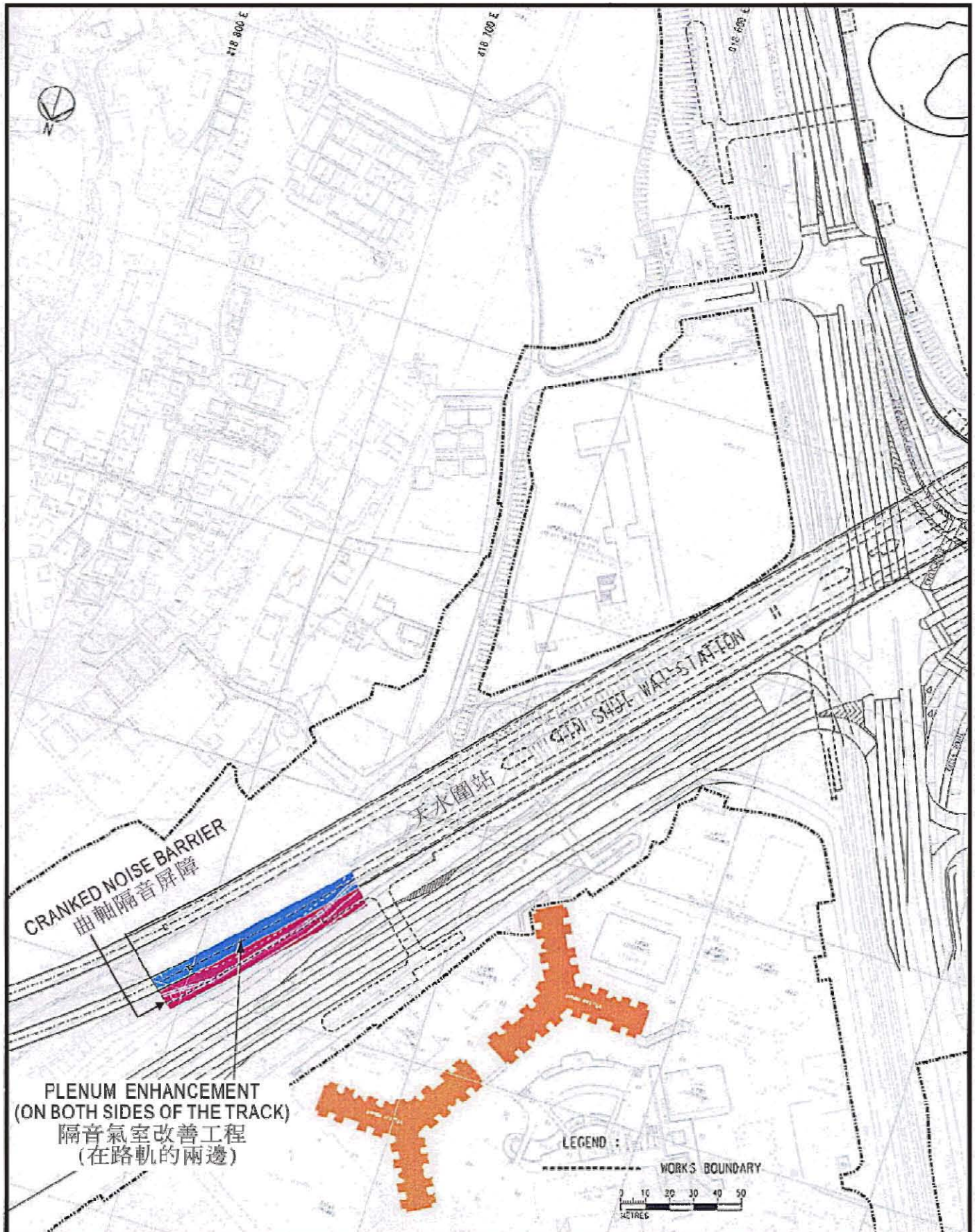
Figure 10 - Cranked Noise Barrier and Plenum Enhancement at the Tin Shui Wai Station 圖十一天水圍站的曲軸隔音屏障及隔音氣室的改善工程
