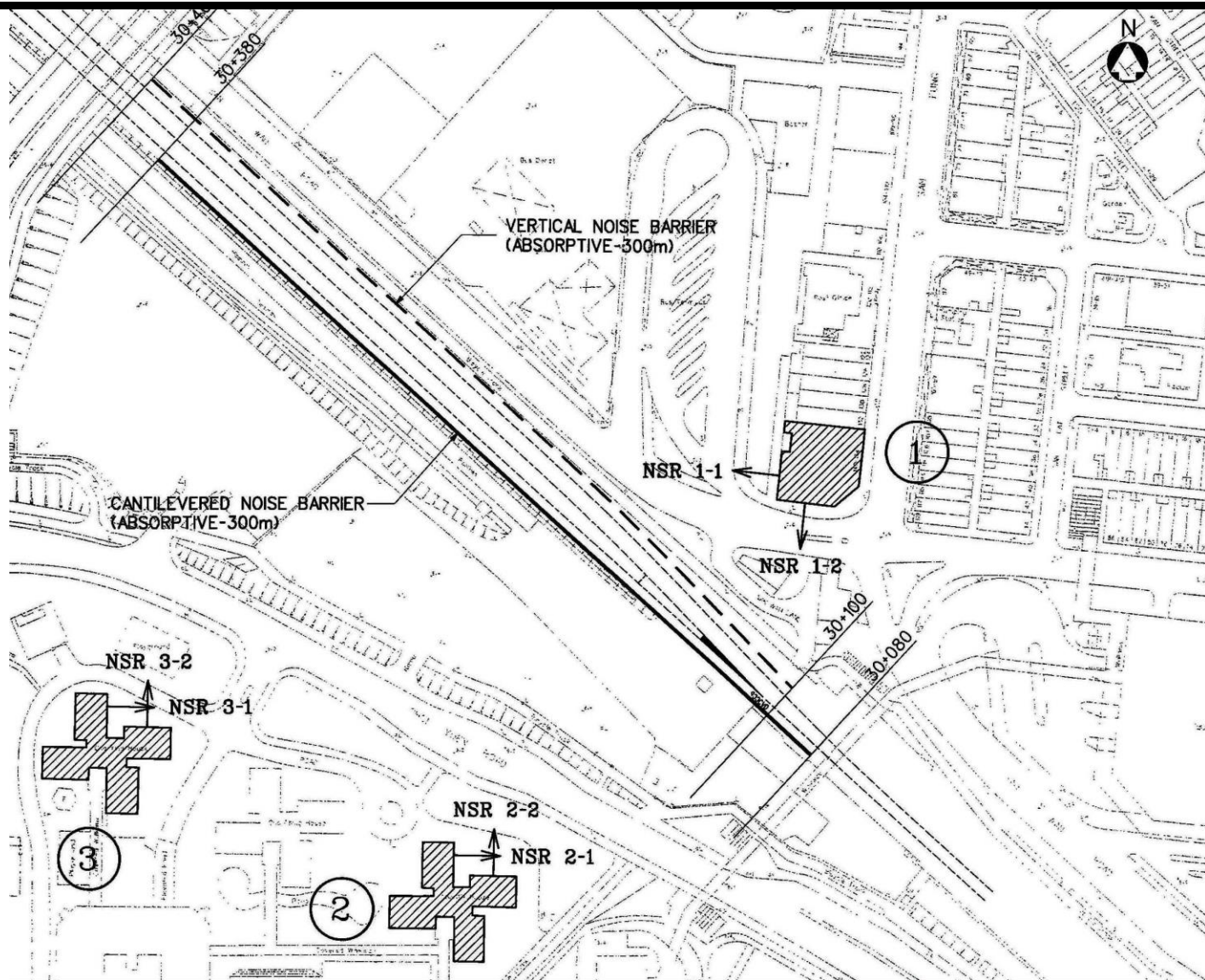
Figure 2 - Sheung Shui to Lok Ma Chau Spur Line (上水至落馬洲支線) 圖二 - 條例 2.5 所指之隔音屏障位置 Locations of Noise Barriers as described in Condition 2.5 of the Permit Reproduced from Drawing No. 7.2b of (Volume 5 of 5) of the EIA Report (Register No.: AEIAR-052/2002) 摘自環評報告第五冊圖 7.2b (登記冊編號: AEIAR-052/2002)
