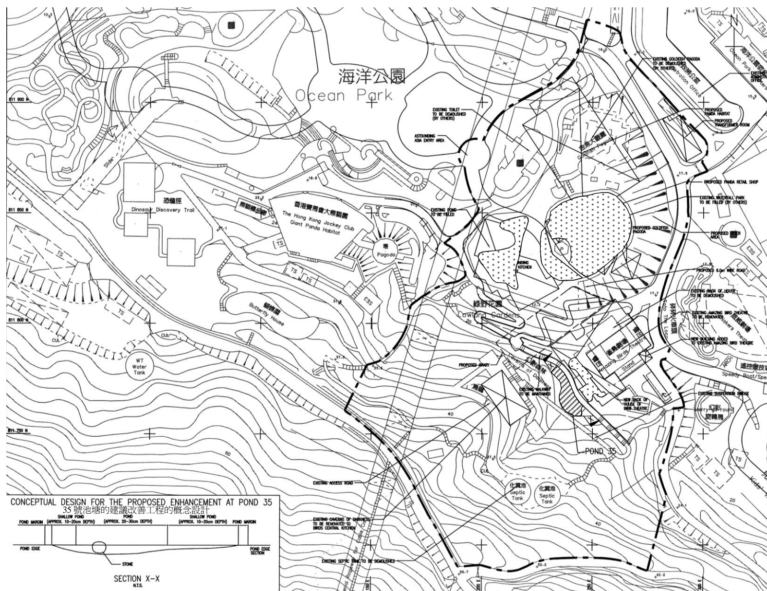
Figure 5: Existing Fresh Water Pond at Lowland 圖 5 : 低地現有淡水池塘
